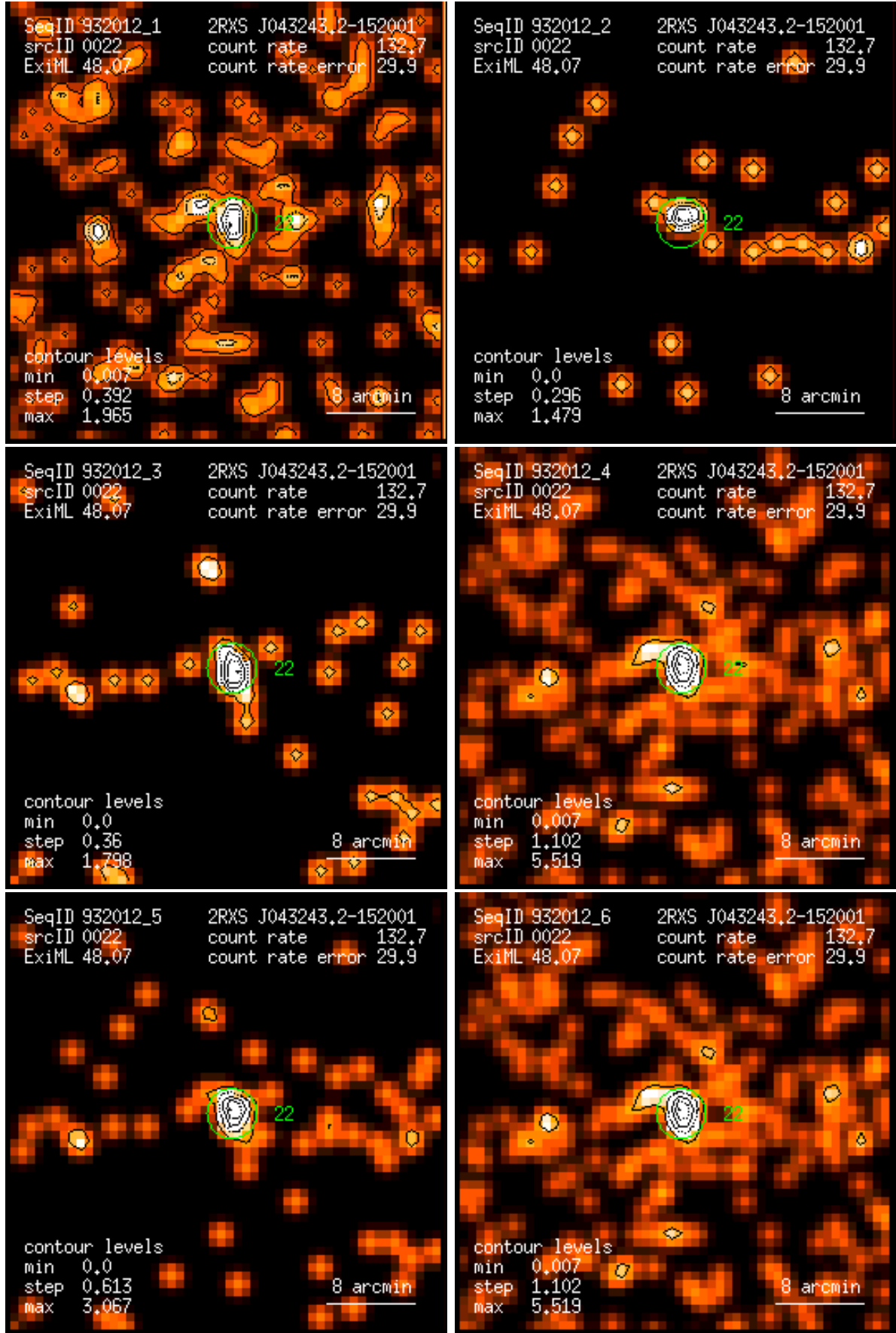
Figure 22: RASS 932012: detection 0022: band rate images, Gaussian filter: (1) PSPC channels 11 – 41, (2) 52 – 90, (3) 91 – 201, (4) 11 – 235, (5) 52 – 201, (6) 11 – 201. Broad band rates in counts/ks. Band rate contour levels in counts/ks/arcmin 2 .
