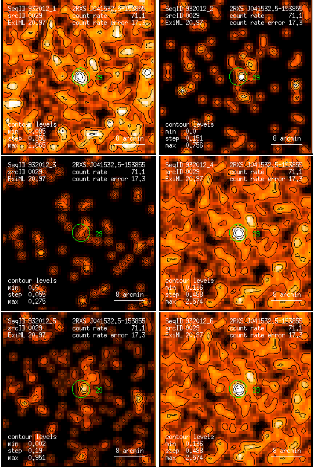
Figure 29: RASS 932012: detection 0029: band rate images, Gaussian filter: (1) PSPC channels 11 – 41, (2) 52 – 90, (3) 91 – 201, (4) 11 – 235, (5) 52 – 201, (6) 11 – 201. Broad band rates in counts/ks. Band rate contour levels in counts/ks/arcmin 2 .
