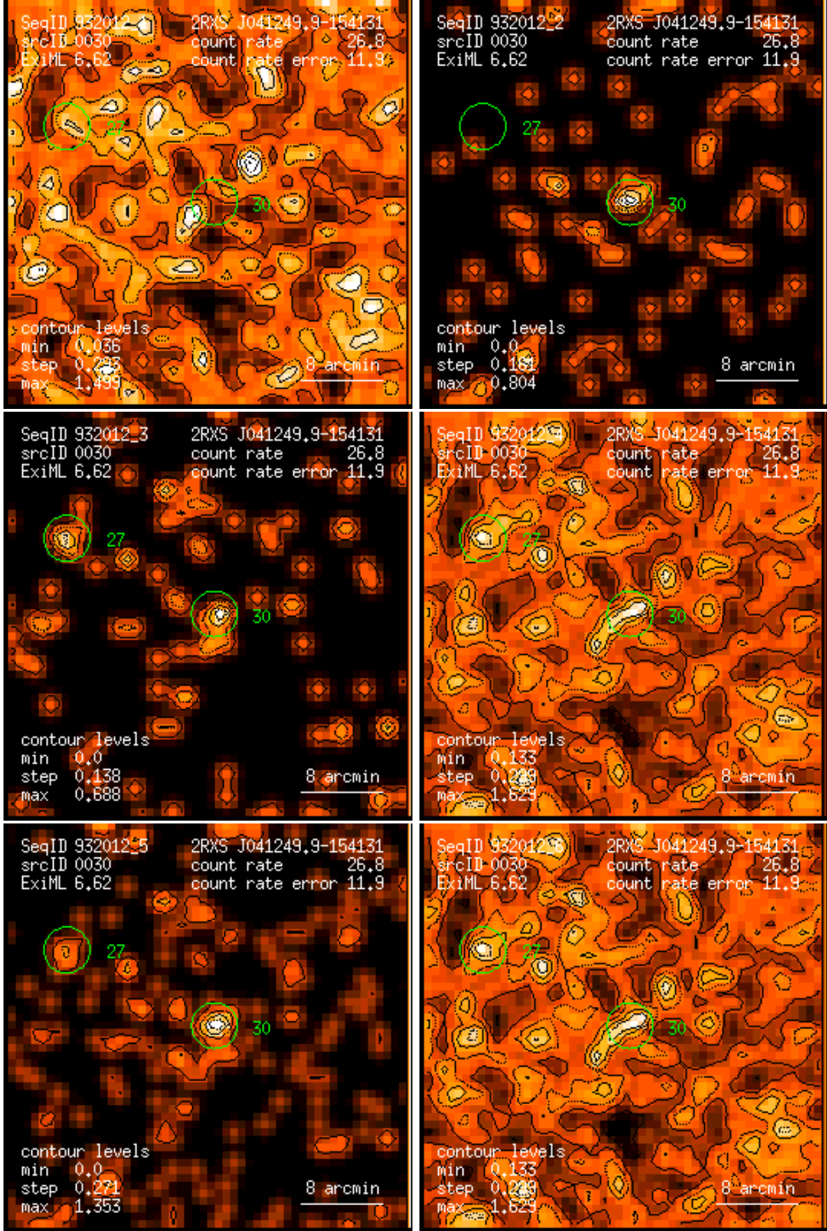
Figure 30: RASS 932012: detection 0030: band rate images, Gaussian filter: (1) PSPC channels 11 – 41, (2) 52 – 90, (3) 91 – 201, (4) 11 – 235, (5) 52 – 201, (6) 11 – 201. Broad band rates in counts/ks. Band rate contour levels in counts/ks/arcmin 2 .
