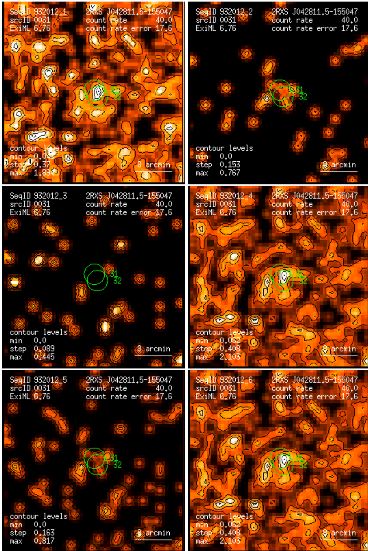
Figure 31: RASS 932012: detection 0031: band rate images, Gaussian filter: (1) PSPC channels 11 – 41, (2) 52 – 90, (3) 91 – 201, (4) 11 – 235, (5) 52 – 201, (6) 11 – 201. Broad band rates in counts/ks. Band rate contour levels in counts/ks/arcmin 2 .
