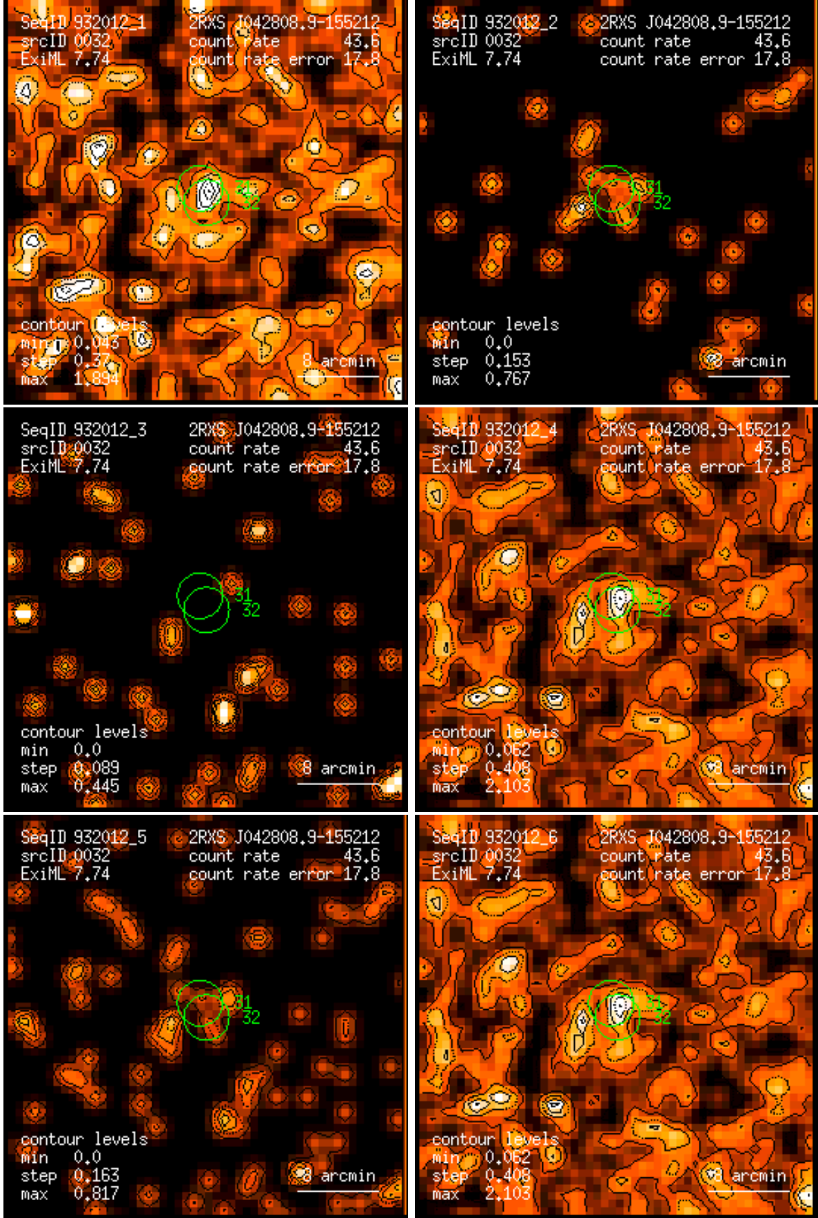
Figure 32: RASS 932012: detection 0032: band rate images, Gaussian filter: (1) PSPC channels 11 – 41, (2) 52 – 90, (3) 91 – 201, (4) 11 – 235, (5) 52 – 201, (6) 11 – 201. Broad band rates in counts/ks. Band rate contour levels in counts/ks/arcmin 2 .
