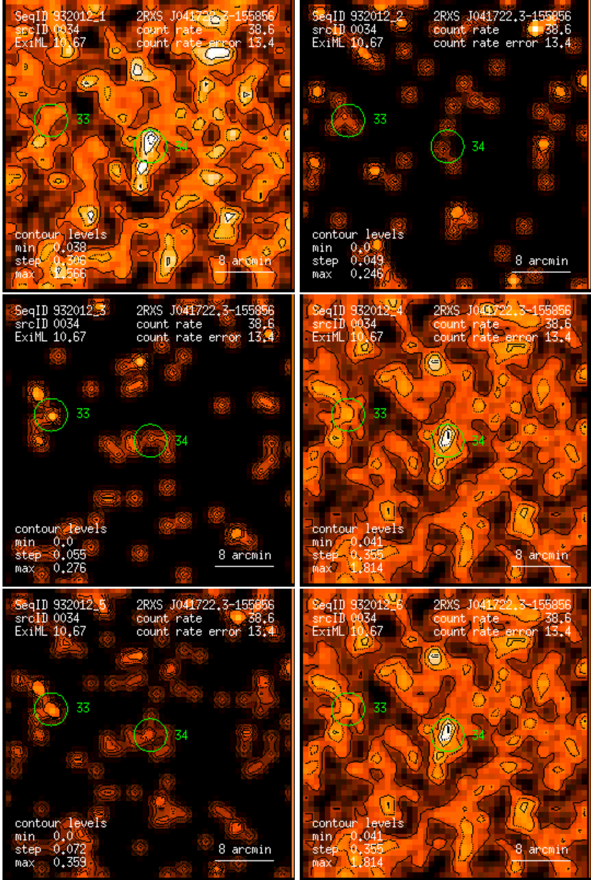
Figure 34: RASS 932012: detection 0034: band rate images, Gaussian filter: (1) PSPC channels 11 – 41, (2) 52 – 90, (3) 91 – 201, (4) 11 – 235, (5) 52 – 201, (6) 11 – 201. Broad band rates in counts/ks. Band rate contour levels in counts/ks/arcmin 2 .
