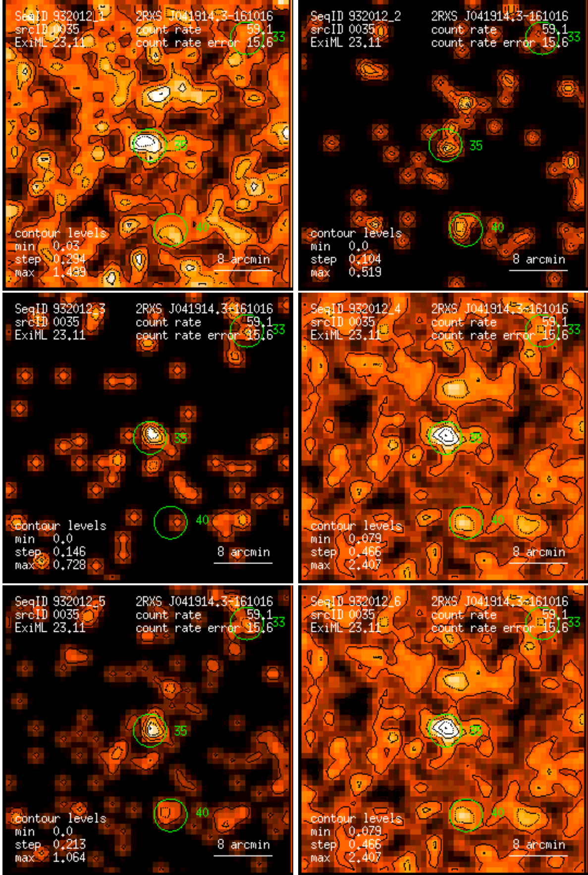
Figure 35: RASS 932012: detection 0035: band rate images, Gaussian filter: (1) PSPC channels 11 – 41, (2) 52 – 90, (3) 91 – 201, (4) 11 – 235, (5) 52 – 201, (6) 11 – 201. Broad band rates in counts/ks. Band rate contour levels in counts/ks/arcmin 2 .
