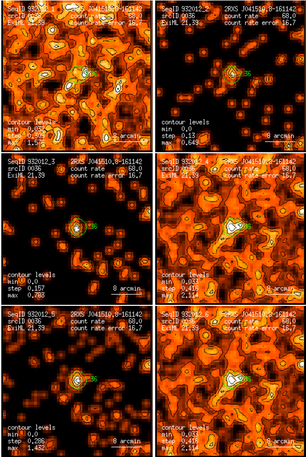
Figure 36: RASS 932012: detection 0036: band rate images, Gaussian filter: (1) PSPC channels 11 – 41, (2) 52 – 90, (3) 91 – 201, (4) 11 – 235, (5) 52 – 201, (6) 11 – 201. Broad band rates in counts/ks. Band rate contour levels in counts/ks/arcmin 2 .
