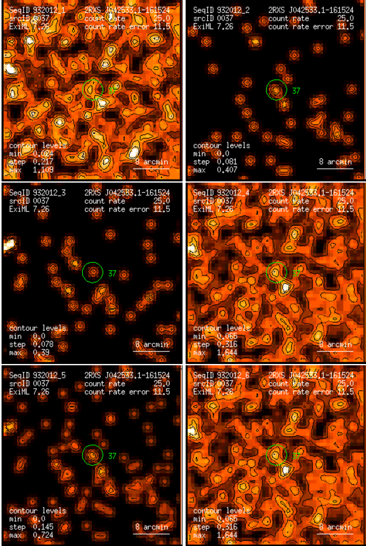
Figure 37: RASS 932012: detection 0037: band rate images, Gaussian filter: (1) PSPC channels 11 – 41, (2) 52 – 90, (3) 91 – 201, (4) 11 – 235, (5) 52 – 201, (6) 11 – 201. Broad band rates in counts/ks. Band rate contour levels in counts/ks/arcmin 2 .
