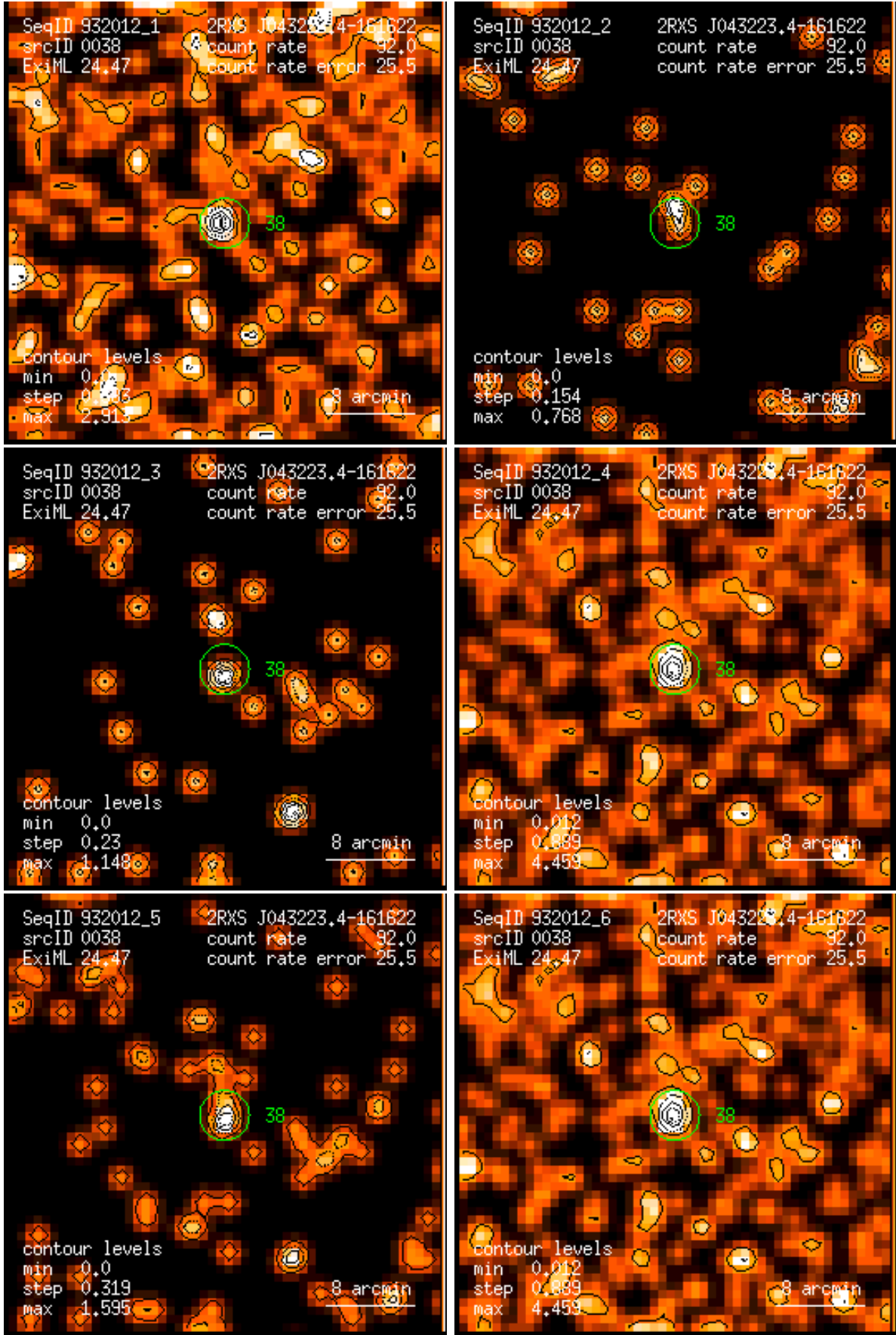
Figure 38: RASS 932012: detection 0038: band rate images, Gaussian filter: (1) PSPC channels 11 – 41, (2) 52 – 90, (3) 91 – 201, (4) 11 – 235, (5) 52 – 201, (6) 11 – 201. Broad band rates in counts/ks. Band rate contour levels in counts/ks/arcmin 2 .
