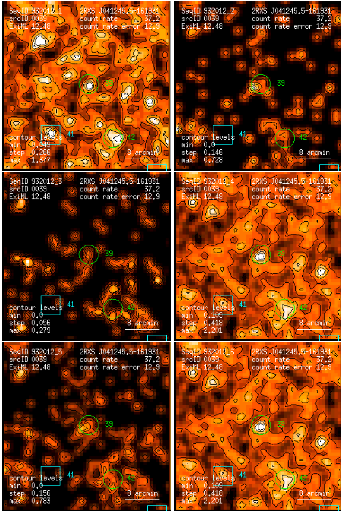
Figure 39: RASS 932012: detection 0039: band rate images, Gaussian filter: (1) PSPC channels 11 – 41, (2) 52 – 90, (3) 91 – 201, (4) 11 – 235, (5) 52 – 201, (6) 11 – 201. Broad band rates in counts/ks. Band rate contour levels in counts/ks/arcmin 2 .
