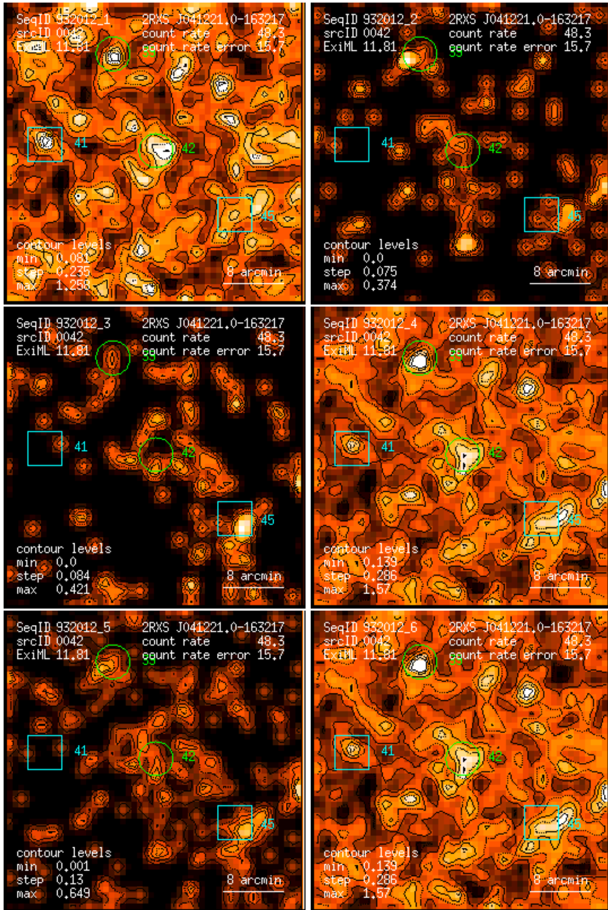
Figure 42: RASS 932012: detection 0042: band rate images, Gaussian filter: (1) PSPC channels 11 – 41, (2) 52 – 90, (3) 91 – 201, (4) 11 – 235, (5) 52 – 201, (6) 11 – 201. Broad band rates in counts/ks. Band rate contour levels in counts/ks/arcmin 2 .
