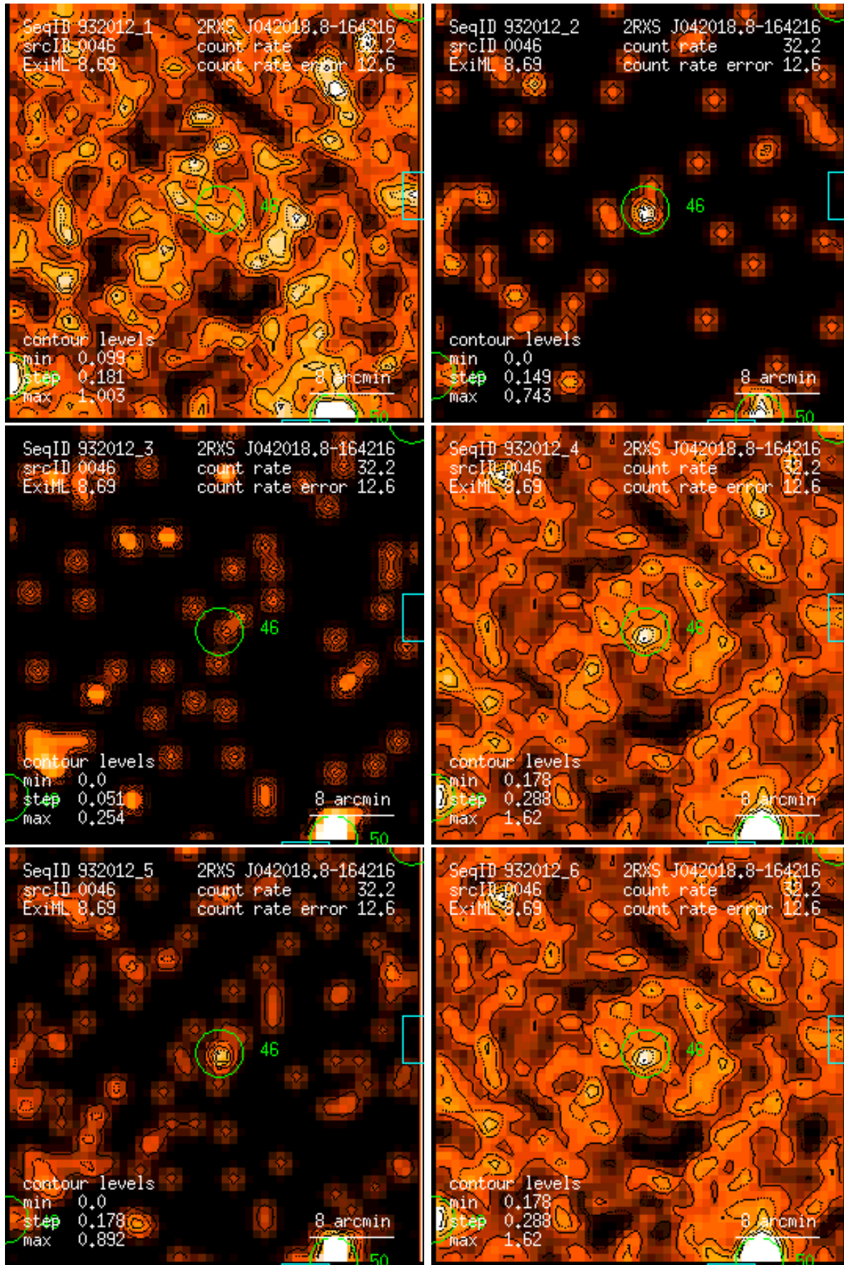
Figure 46: RASS 932012: detection 0046: band rate images, Gaussian filter: (1) PSPC channels 11 – 41, (2) 52 – 90, (3) 91 – 201, (4) 11 – 235, (5) 52 – 201, (6) 11 – 201. Broad band rates in counts/ks. Band rate contour levels in counts/ks/arcmin 2 .
