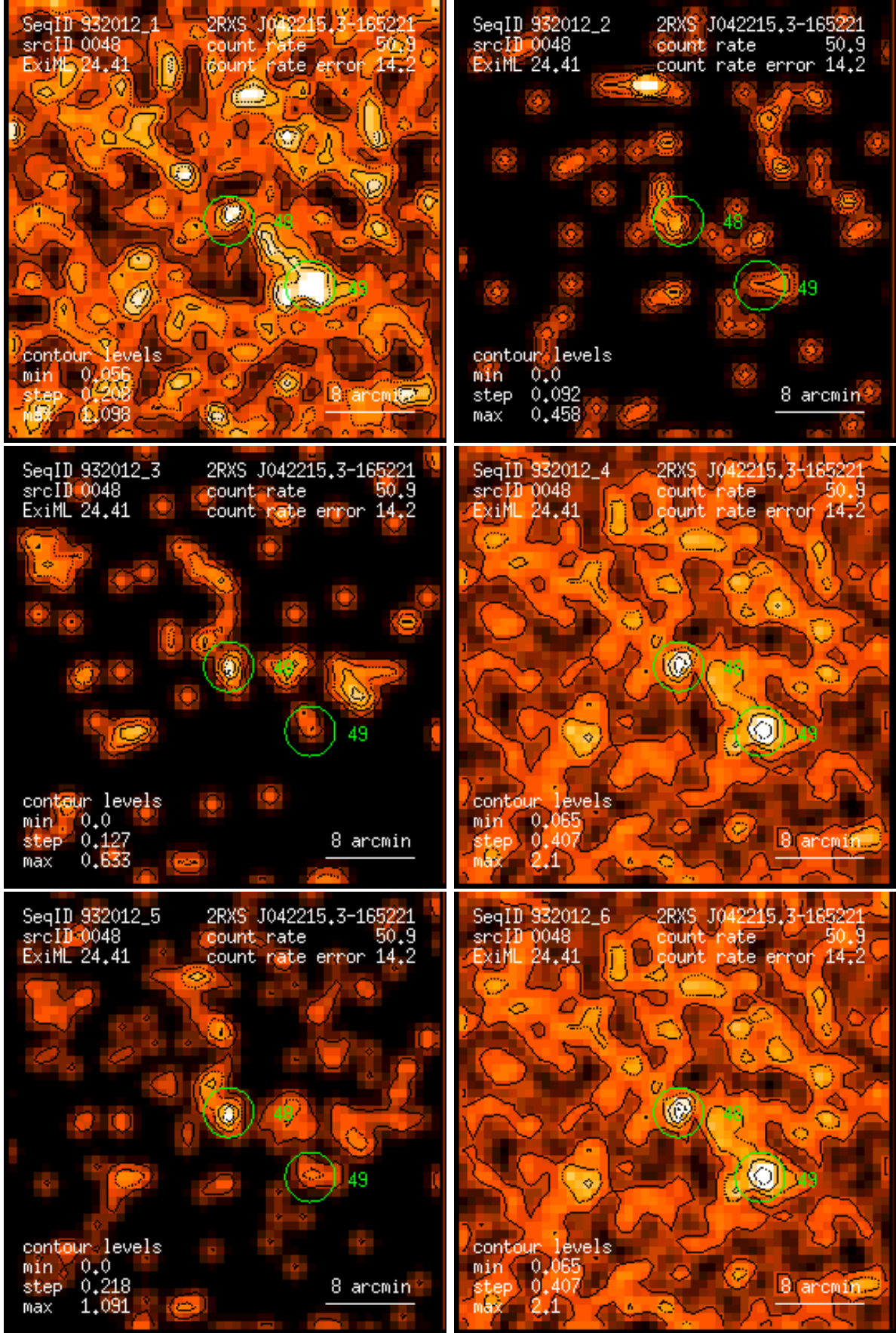
Figure 48: RASS 932012: detection 0048: band rate images, Gaussian filter: (1) PSPC channels 11 – 41, (2) 52 – 90, (3) 91 – 201, (4) 11 – 235, (5) 52 – 201, (6) 11 – 201. Broad band rates in counts/ks. Band rate contour levels in counts/ks/arcmin 2 .
