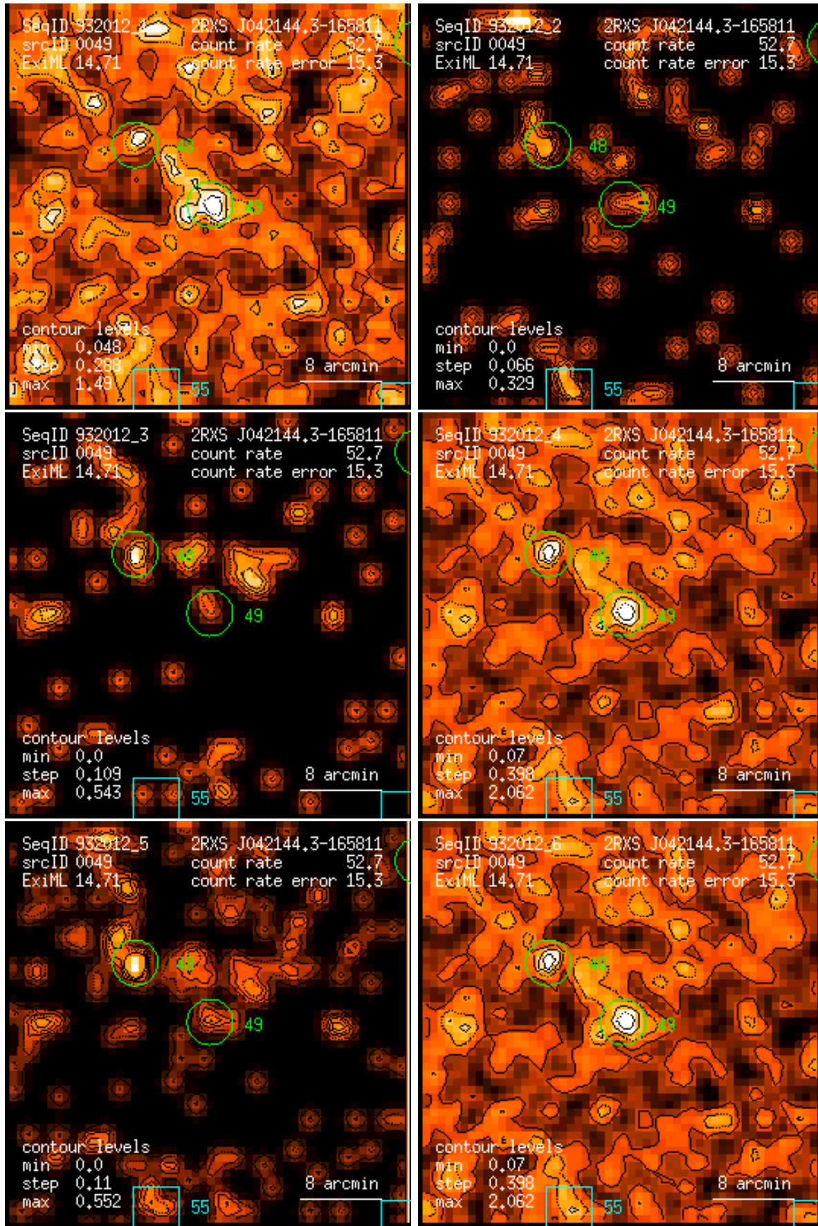
Figure 49: RASS 932012: detection 0049: band rate images, Gaussian filter: (1) PSPC channels 11 – 41, (2) 52 – 90, (3) 91 – 201, (4) 11 – 235, (5) 52 – 201, (6) 11 – 201. Broad band rates in counts/ks. Band rate contour levels in counts/ks/arcmin 2 .
