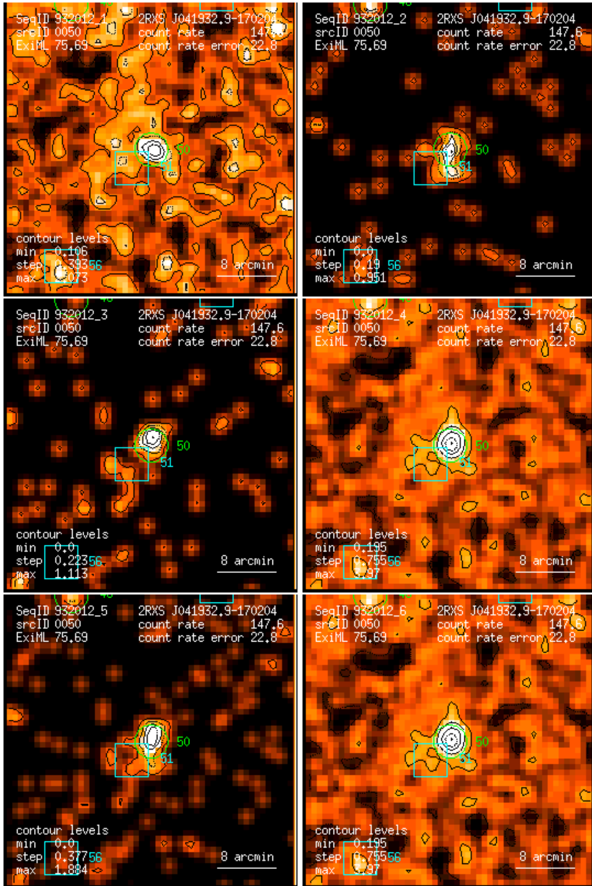
Figure 50: RASS 932012: detection 0050: band rate images, Gaussian filter: (1) PSPC channels 11 – 41, (2) 52 – 90, (3) 91 – 201, (4) 11 – 235, (5) 52 – 201, (6) 11 – 201. Broad band rates in counts/ks. Band rate contour levels in counts/ks/arcmin 2 .
