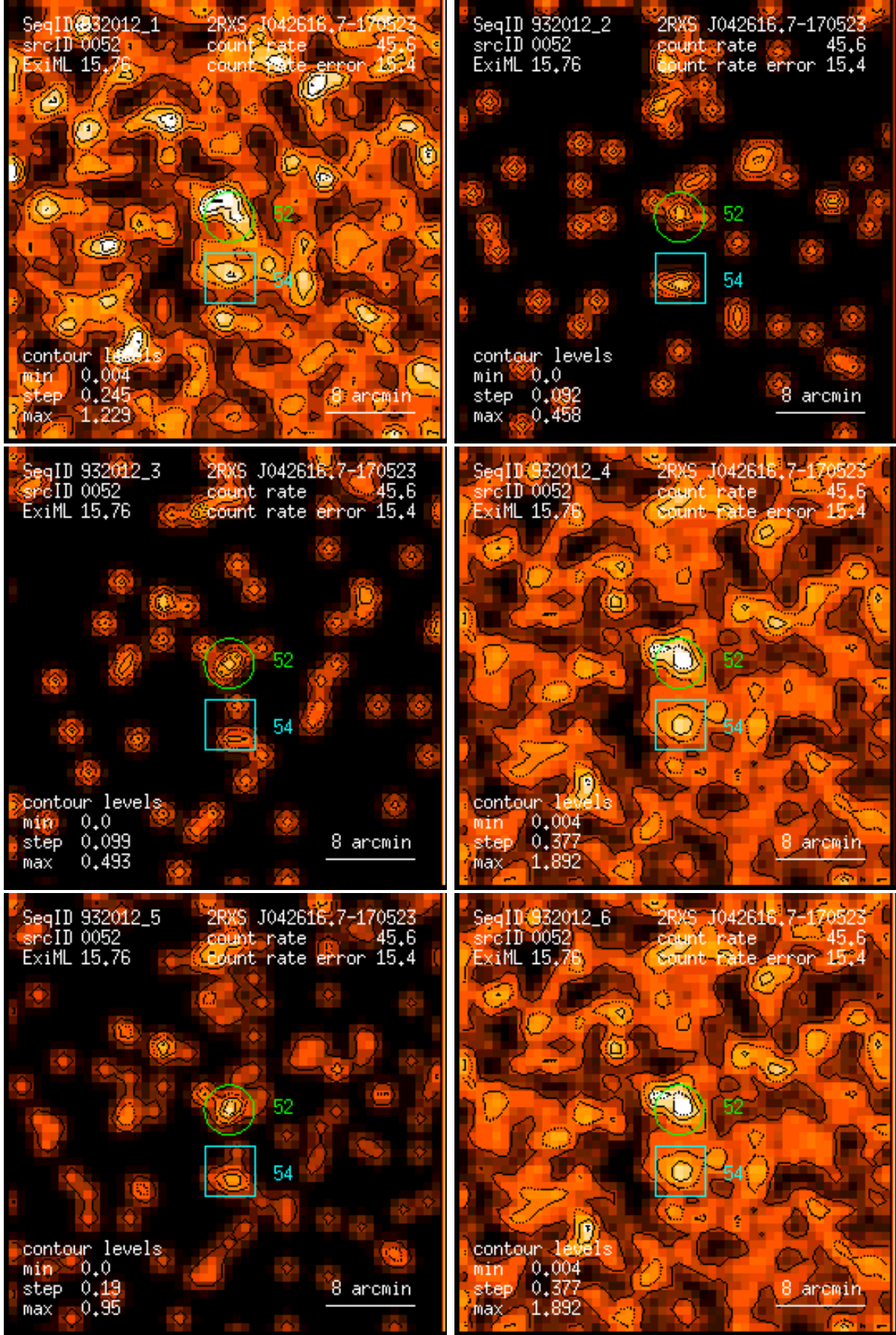
Figure 52: RASS 932012: detection 0052: band rate images, Gaussian filter: (1) PSPC channels 11 – 41, (2) 52 – 90, (3) 91 – 201, (4) 11 – 235, (5) 52 – 201, (6) 11 – 201. Broad band rates in counts/ks. Band rate contour levels in counts/ks/arcmin 2 .
