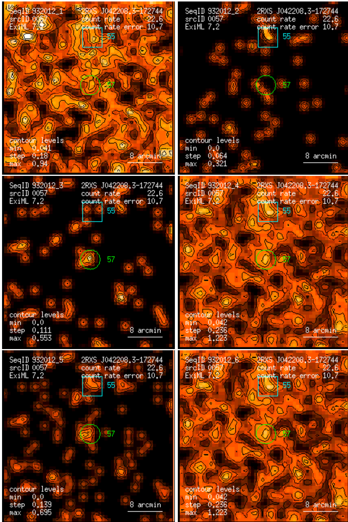
Figure 57: RASS 932012: detection 0057: band rate images, Gaussian filter: (1) PSPC channels 11 – 41, (2) 52 – 90, (3) 91 – 201, (4) 11 – 235, (5) 52 – 201, (6) 11 – 201. Broad band rates in counts/ks. Band rate contour levels in counts/ks/arcmin 2 .
