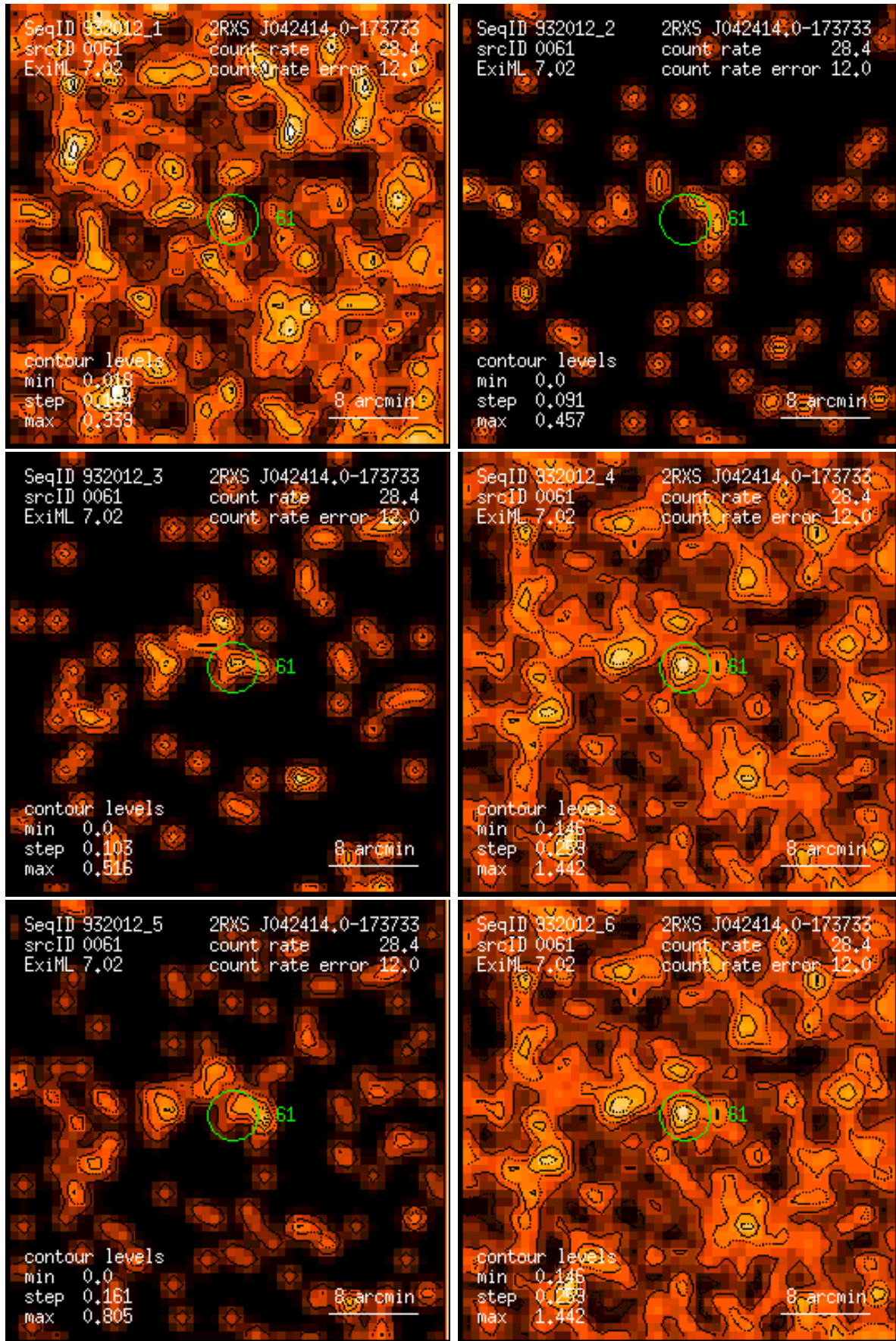
Figure 61: RASS 932012: detection 0061: band rate images, Gaussian filter: (1) PSPC channels 11 – 41, (2) 52 – 90, (3) 91 – 201, (4) 11 – 235, (5) 52 – 201, (6) 11 – 201. Broad band rates in counts/ks. Band rate contour levels in counts/ks/arcmin 2 .
