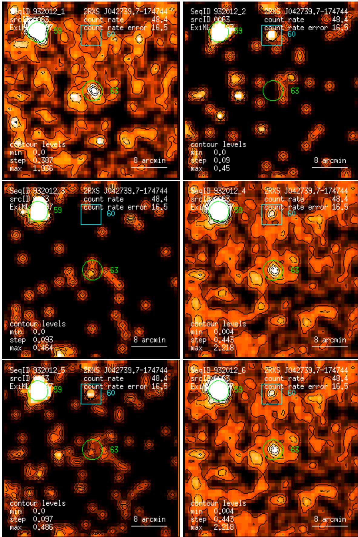
Figure 63: RASS 932012: detection 0063: band rate images, Gaussian filter: (1) PSPC channels 11 – 41, (2) 52 – 90, (3) 91 – 201, (4) 11 – 235, (5) 52 – 201, (6) 11 – 201. Broad band rates in counts/ks. Band rate contour levels in counts/ks/arcmin 2 .
