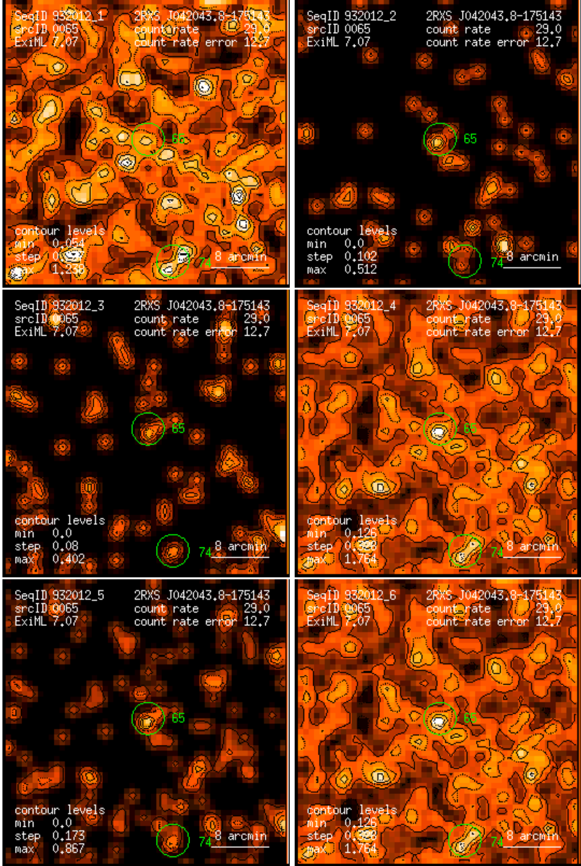
Figure 65: RASS 932012: detection 0065: band rate images, Gaussian filter: (1) PSPC channels 11 – 41, (2) 52 – 90, (3) 91 – 201, (4) 11 – 235, (5) 52 – 201, (6) 11 – 201. Broad band rates in counts/ks. Band rate contour levels in counts/ks/arcmin 2 .
