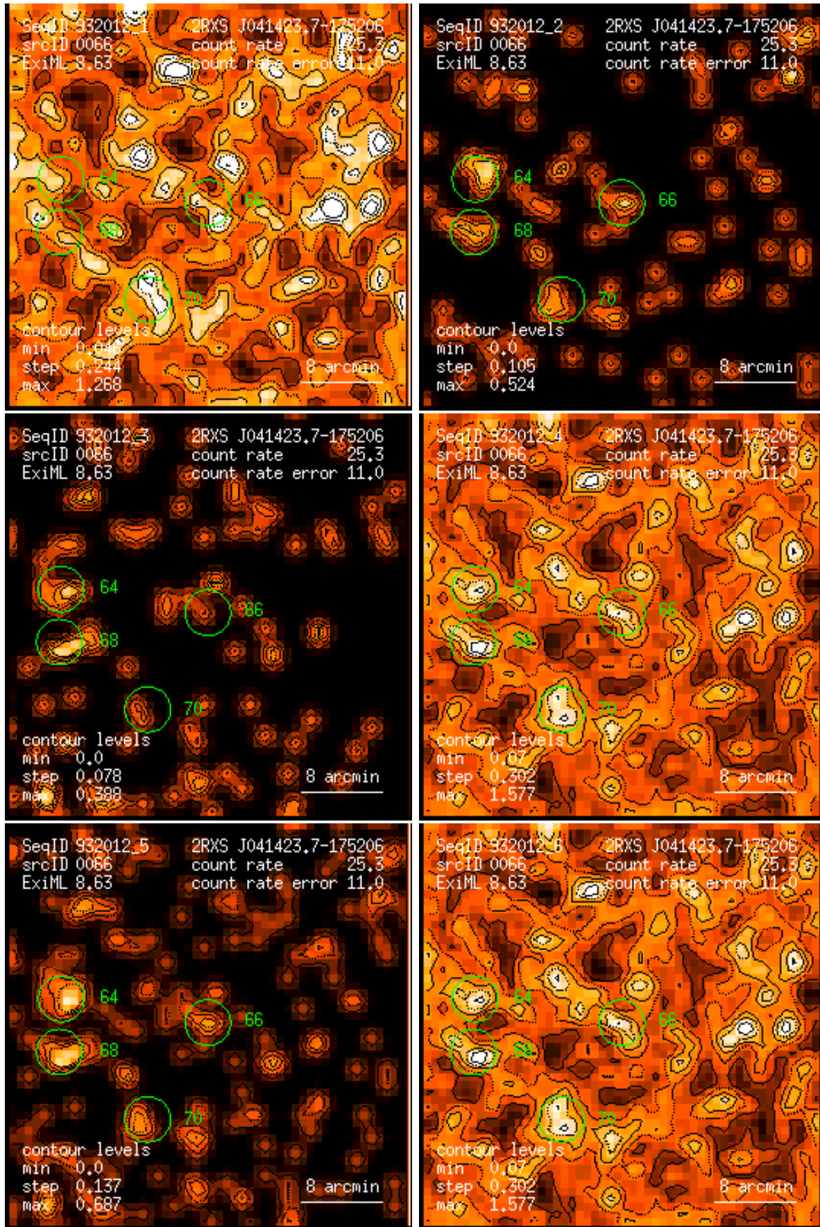
Figure 66: RASS 932012: detection 0066: band rate images, Gaussian filter: (1) PSPC channels 11 – 41, (2) 52 – 90, (3) 91 – 201, (4) 11 – 235, (5) 52 – 201, (6) 11 – 201. Broad band rates in counts/ks. Band rate contour levels in counts/ks/arcmin 2 .
