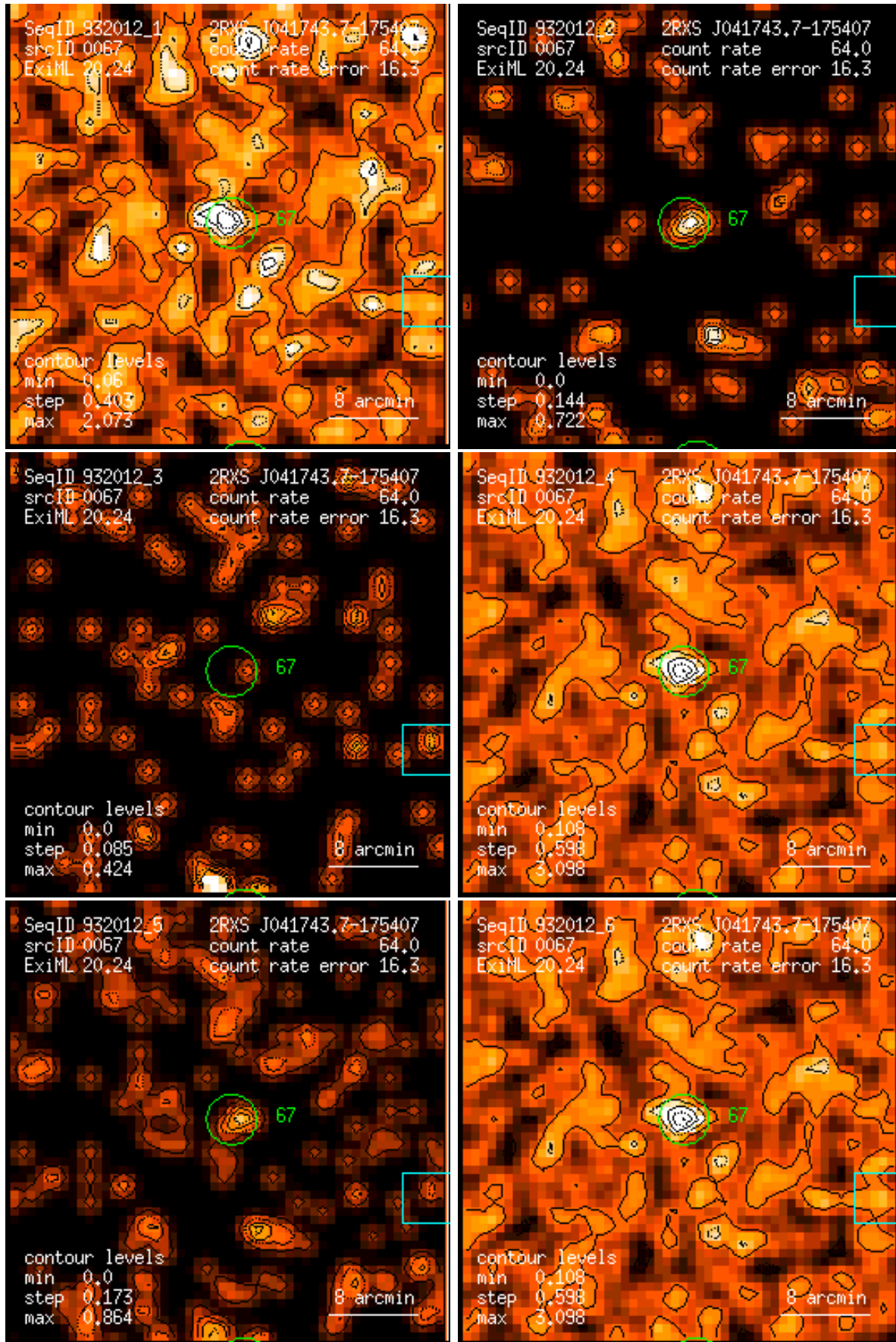
Figure 67: RASS 932012: detection 0067: band rate images, Gaussian filter: (1) PSPC channels 11 – 41, (2) 52 – 90, (3) 91 – 201, (4) 11 – 235, (5) 52 – 201, (6) 11 – 201. Broad band rates in counts/ks. Band rate contour levels in counts/ks/arcmin 2 .
