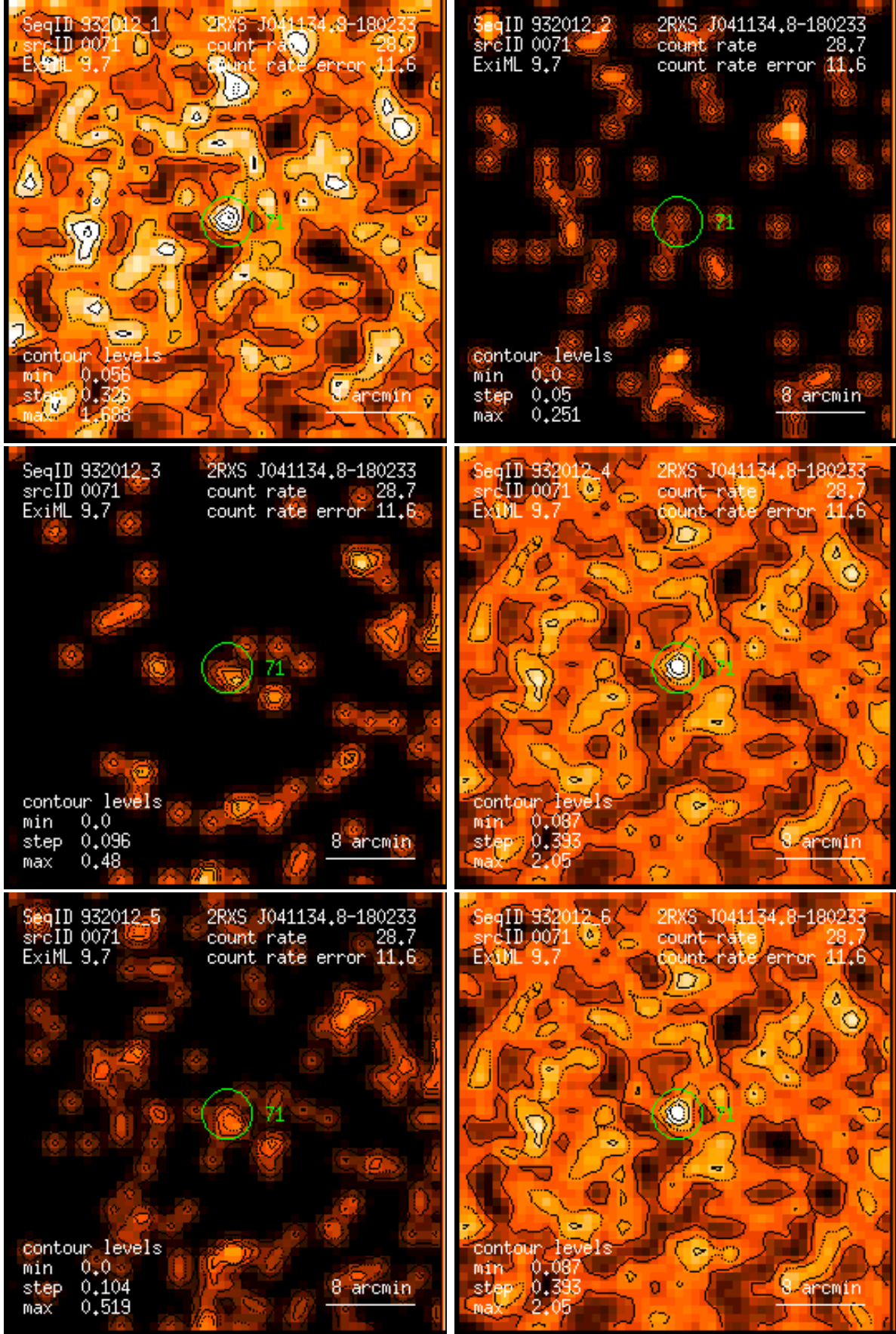
Figure 71: RASS 932012: detection 0071: band rate images, Gaussian filter: (1) PSPC channels 11 – 41, (2) 52 – 90, (3) 91 – 201, (4) 11 – 235, (5) 52 – 201, (6) 11 – 201. Broad band rates in counts/ks. Band rate contour levels in counts/ks/arcmin 2 .
