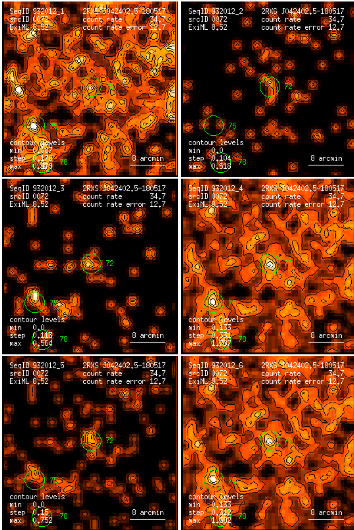
Figure 72: RASS 932012: detection 0072: band rate images, Gaussian filter: (1) PSPC channels 11 – 41, (2) 52 – 90, (3) 91 – 201, (4) 11 – 235, (5) 52 – 201, (6) 11 – 201. Broad band rates in counts/ks. Band rate contour levels in counts/ks/arcmin 2 .
