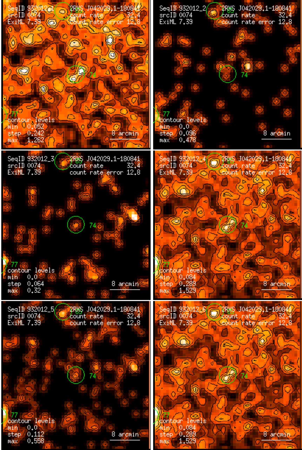
Figure 74: RASS 932012: detection 0074: band rate images, Gaussian filter: (1) PSPC channels 11 – 41, (2) 52 – 90, (3) 91 – 201, (4) 11 – 235, (5) 52 – 201, (6) 11 – 201. Broad band rates in counts/ks. Band rate contour levels in counts/ks/arcmin 2 .
