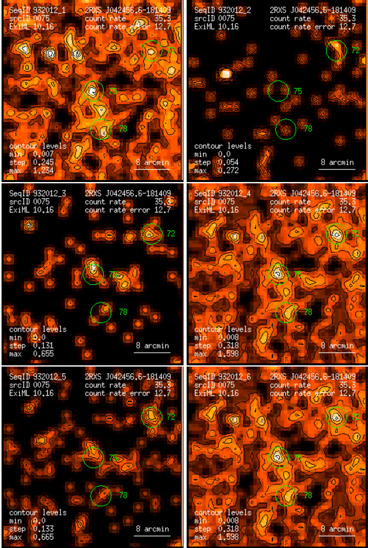
Figure 75: RASS 932012: detection 0075: band rate images, Gaussian filter: (1) PSPC channels 11 – 41, (2) 52 – 90, (3) 91 – 201, (4) 11 – 235, (5) 52 – 201, (6) 11 – 201. Broad band rates in counts/ks. Band rate contour levels in counts/ks/arcmin 2 .
