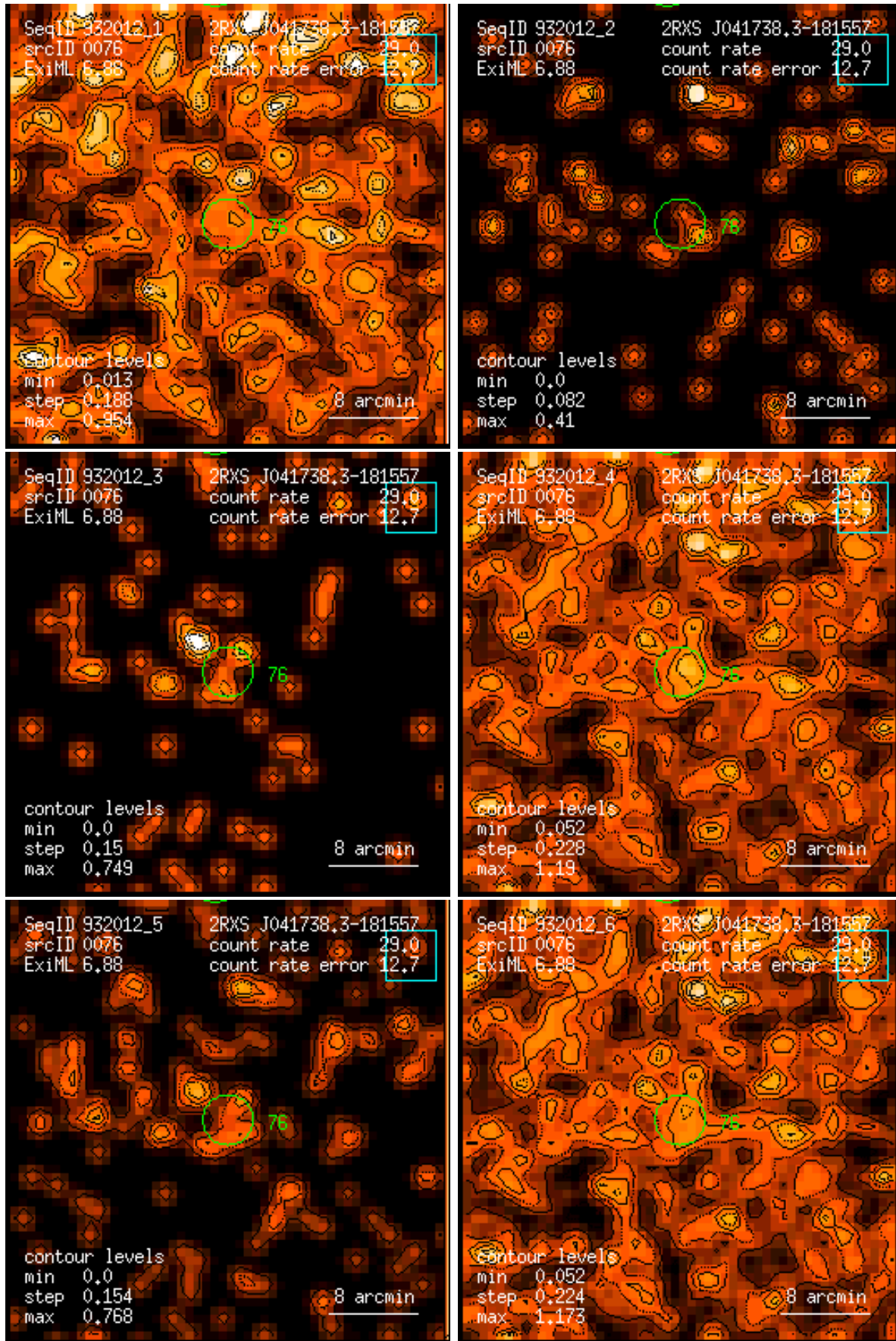
Figure 76: RASS 932012: detection 0076: band rate images, Gaussian filter: (1) PSPC channels 11 – 41, (2) 52 – 90, (3) 91 – 201, (4) 11 – 235, (5) 52 – 201, (6) 11 – 201. Broad band rates in counts/ks. Band rate contour levels in counts/ks/arcmin 2 .
