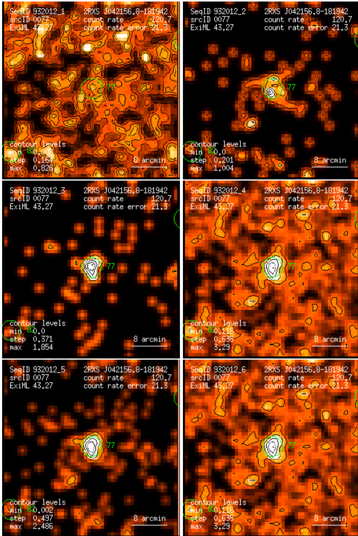
Figure 77: RASS 932012: detection 0077: band rate images, Gaussian filter: (1) PSPC channels 11 – 41, (2) 52 – 90, (3) 91 – 201, (4) 11 – 235, (5) 52 – 201, (6) 11 – 201. Broad band rates in counts/ks. Band rate contour levels in counts/ks/arcmin 2 .
