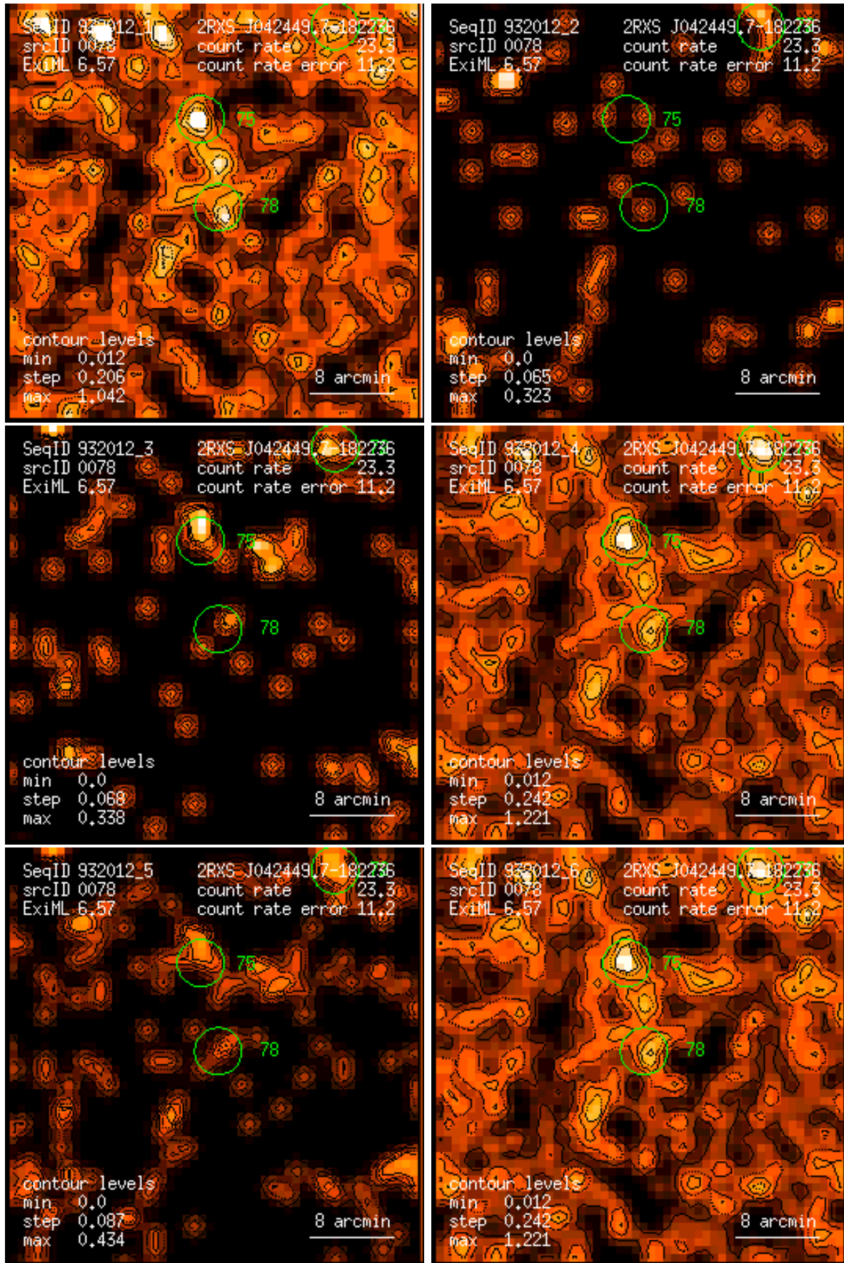
Figure 78: RASS 932012: detection 0078: band rate images, Gaussian filter: (1) PSPC channels 11 – 41, (2) 52 – 90, (3) 91 – 201, (4) 11 – 235, (5) 52 – 201, (6) 11 – 201. Broad band rates in counts/ks. Band rate contour levels in counts/ks/arcmin 2 .
