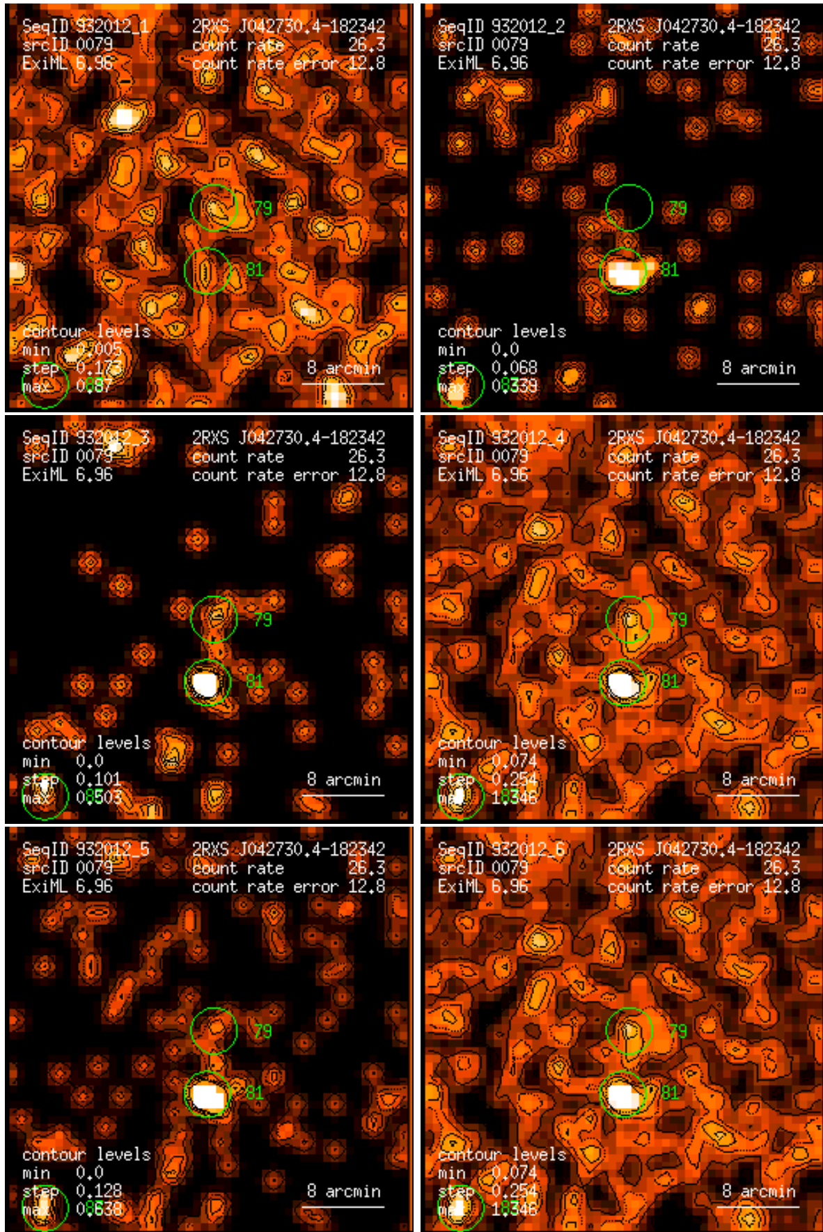
Figure 79: RASS 932012: detection 0079: band rate images, Gaussian filter: (1) PSPC channels 11 – 41, (2) 52 – 90, (3) 91 – 201, (4) 11 – 235, (5) 52 – 201, (6) 11 – 201. Broad band rates in counts/ks. Band rate contour levels in counts/ks/arcmin 2 .
