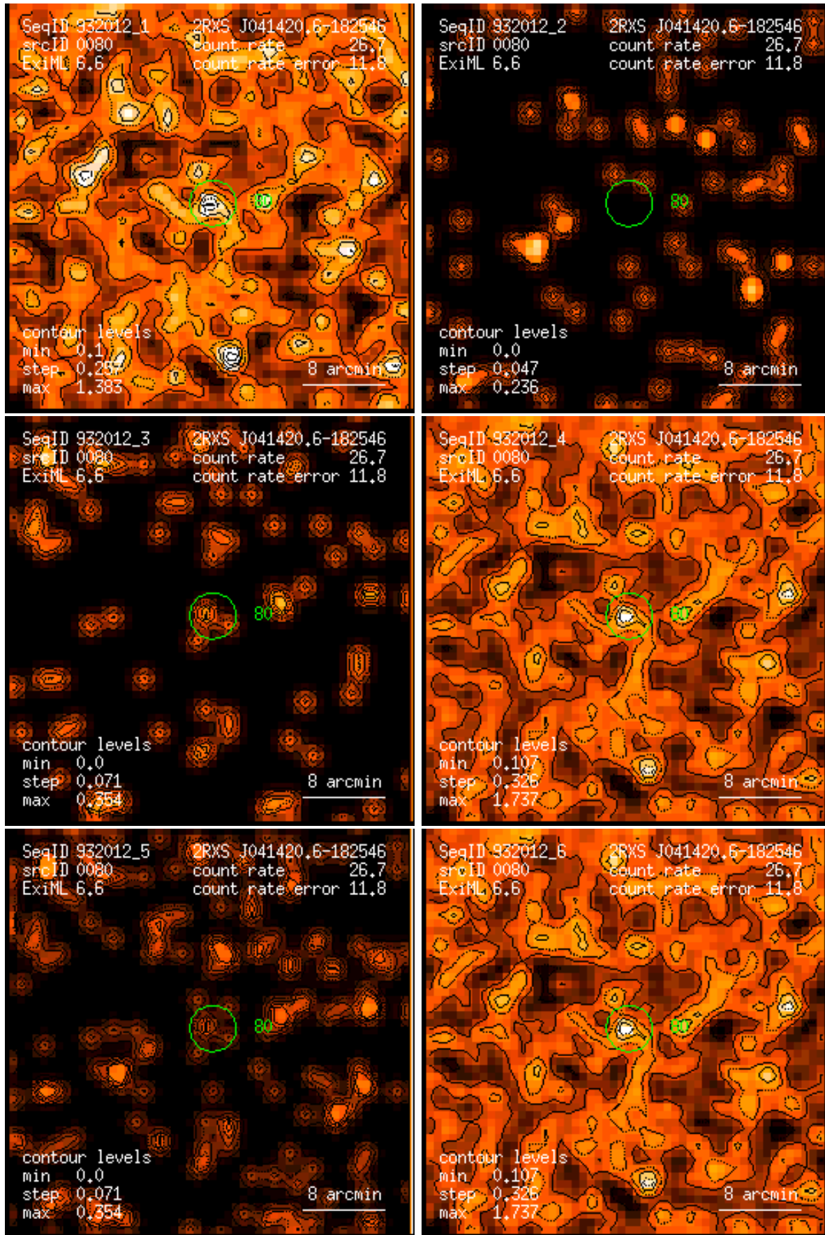
Figure 80: RASS 932012: detection 0080: band rate images, Gaussian filter: (1) PSPC channels 11 – 41, (2) 52 – 90, (3) 91 – 201, (4) 11 – 235, (5) 52 – 201, (6) 11 – 201. Broad band rates in counts/ks. Band rate contour levels in counts/ks/arcmin 2 .
