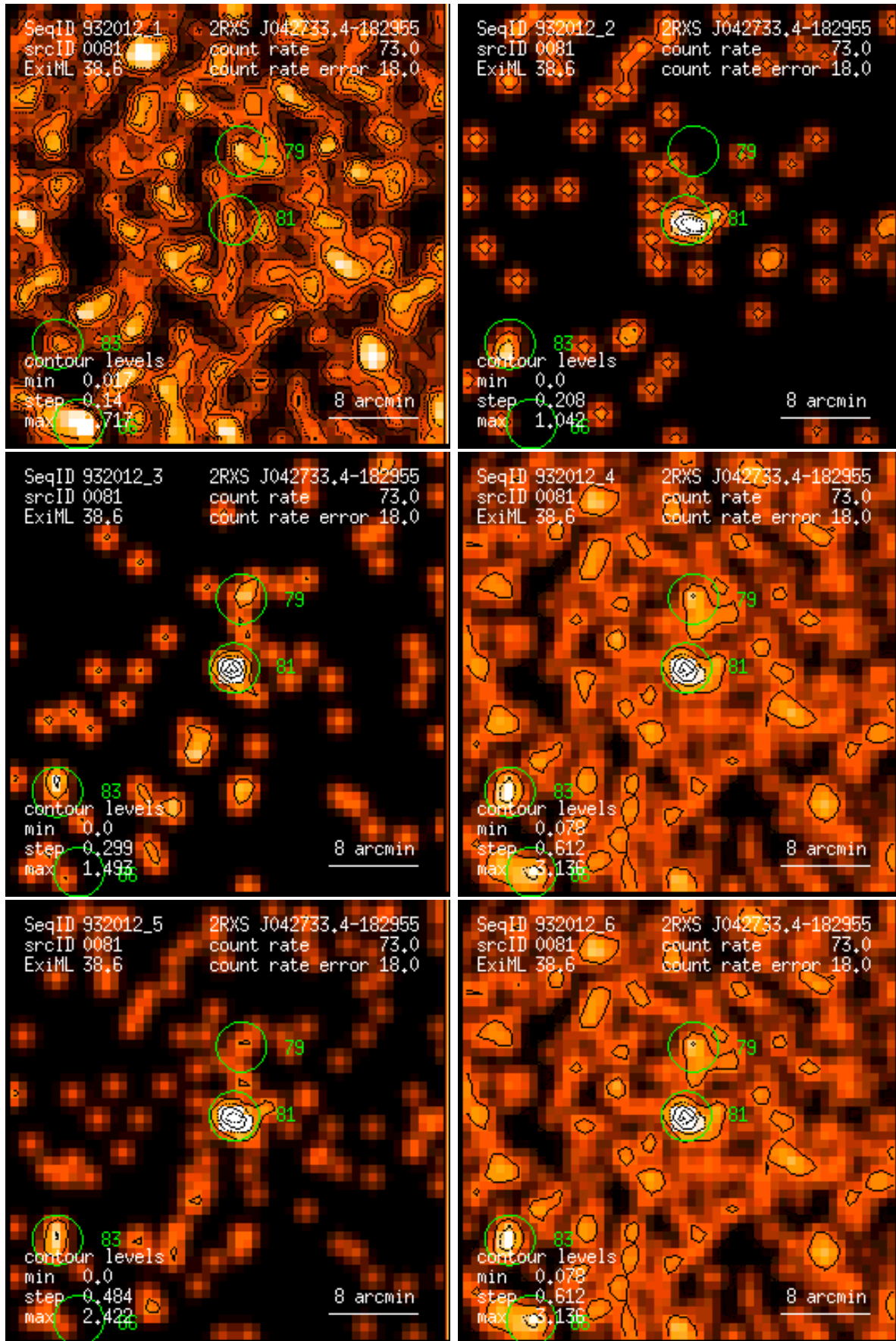
Figure 81: RASS 932012: detection 0081: band rate images, Gaussian filter: (1) PSPC channels 11 – 41, (2) 52 – 90, (3) 91 – 201, (4) 11 – 235, (5) 52 – 201, (6) 11 – 201. Broad band rates in counts/ks. Band rate contour levels in counts/ks/arcmin 2 .
