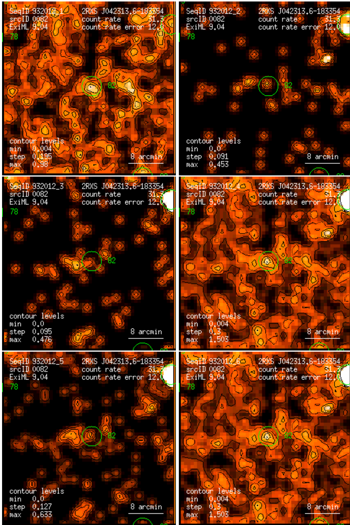
Figure 82: RASS 932012: detection 0082: band rate images, Gaussian filter: (1) PSPC channels 11 – 41, (2) 52 – 90, (3) 91 – 201, (4) 11 – 235, (5) 52 – 201, (6) 11 – 201. Broad band rates in counts/ks. Band rate contour levels in counts/ks/arcmin 2 .
