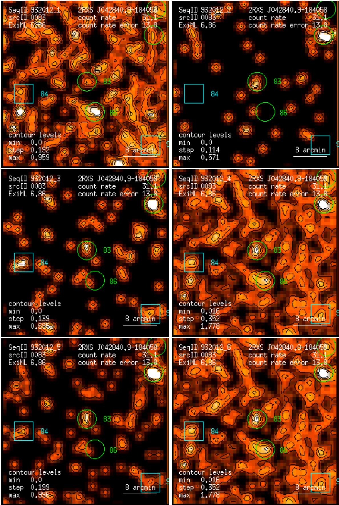
Figure 83: RASS 932012: detection 0083: band rate images, Gaussian filter: (1) PSPC channels 11 – 41, (2) 52 – 90, (3) 91 – 201, (4) 11 – 235, (5) 52 – 201, (6) 11 – 201. Broad band rates in counts/ks. Band rate contour levels in counts/ks/arcmin 2 .
