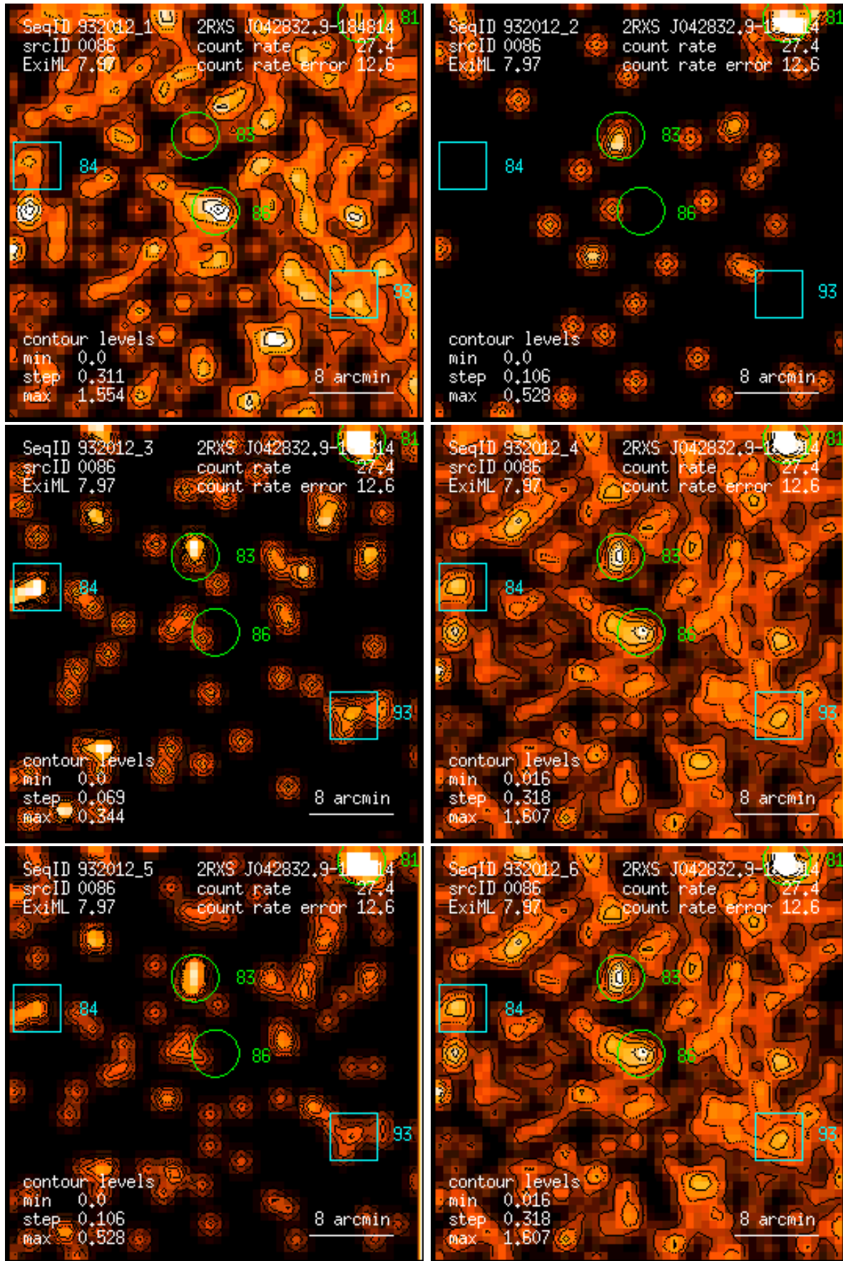
Figure 86: RASS 932012: detection 0086: band rate images, Gaussian filter: (1) PSPC channels 11 – 41, (2) 52 – 90, (3) 91 – 201, (4) 11 – 235, (5) 52 – 201, (6) 11 – 201. Broad band rates in counts/ks. Band rate contour levels in counts/ks/arcmin 2 .
