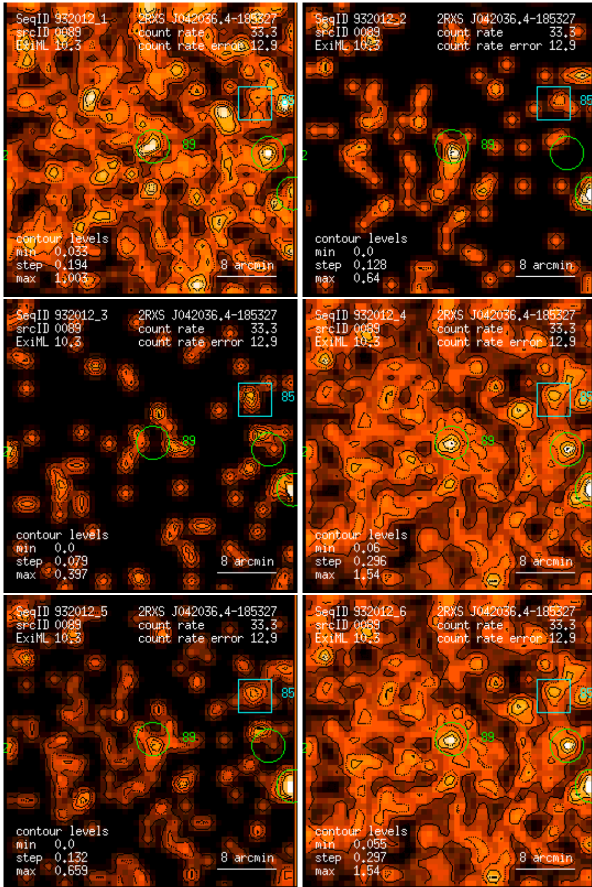
Figure 89: RASS 932012: detection 0089: band rate images, Gaussian filter: (1) PSPC channels 11 – 41, (2) 52 – 90, (3) 91 – 201, (4) 11 – 235, (5) 52 – 201, (6) 11 – 201. Broad band rates in counts/ks. Band rate contour levels in counts/ks/arcmin 2 .
