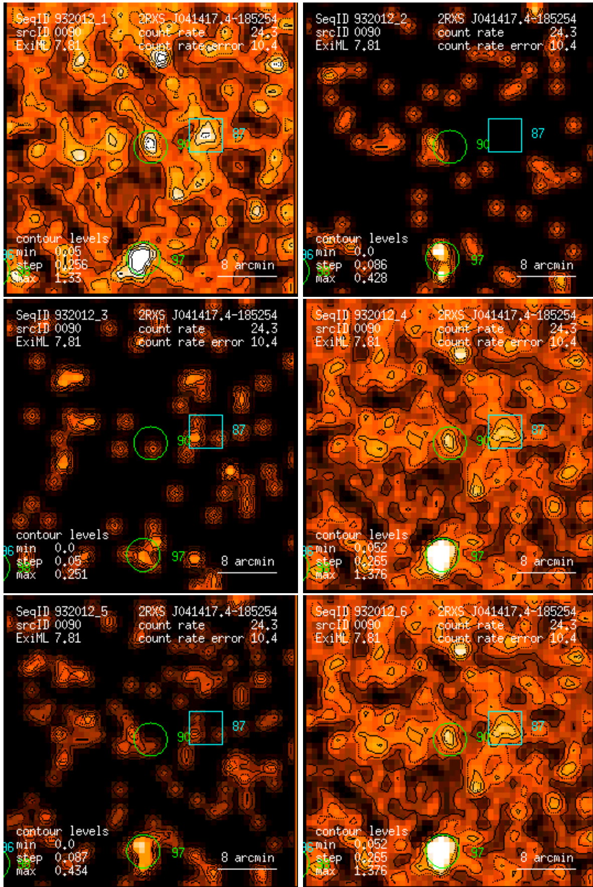
Figure 90: RASS 932012: detection 0090: band rate images, Gaussian filter: (1) PSPC channels 11 – 41, (2) 52 – 90, (3) 91 – 201, (4) 11 – 235, (5) 52 – 201, (6) 11 – 201. Broad band rates in counts/ks. Band rate contour levels in counts/ks/arcmin 2 .
