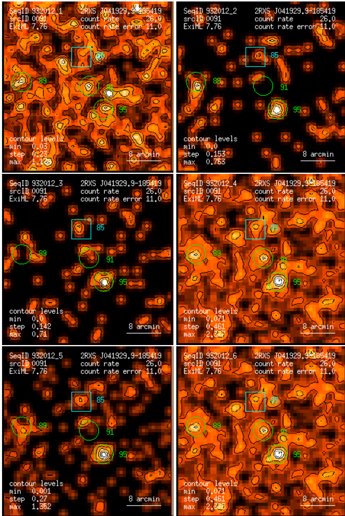
Figure 91: RASS 932012: detection 0091: band rate images, Gaussian filter: (1) PSPC channels 11 – 41, (2) 52 – 90, (3) 91 – 201, (4) 11 – 235, (5) 52 – 201, (6) 11 – 201. Broad band rates in counts/ks. Band rate contour levels in counts/ks/arcmin 2 .
