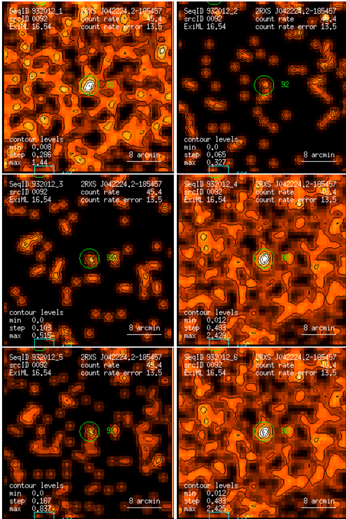
Figure 92: RASS 932012: detection 0092: band rate images, Gaussian filter: (1) PSPC channels 11 – 41, (2) 52 – 90, (3) 91 – 201, (4) 11 – 235, (5) 52 – 201, (6) 11 – 201. Broad band rates in counts/ks. Band rate contour levels in counts/ks/arcmin 2 .
