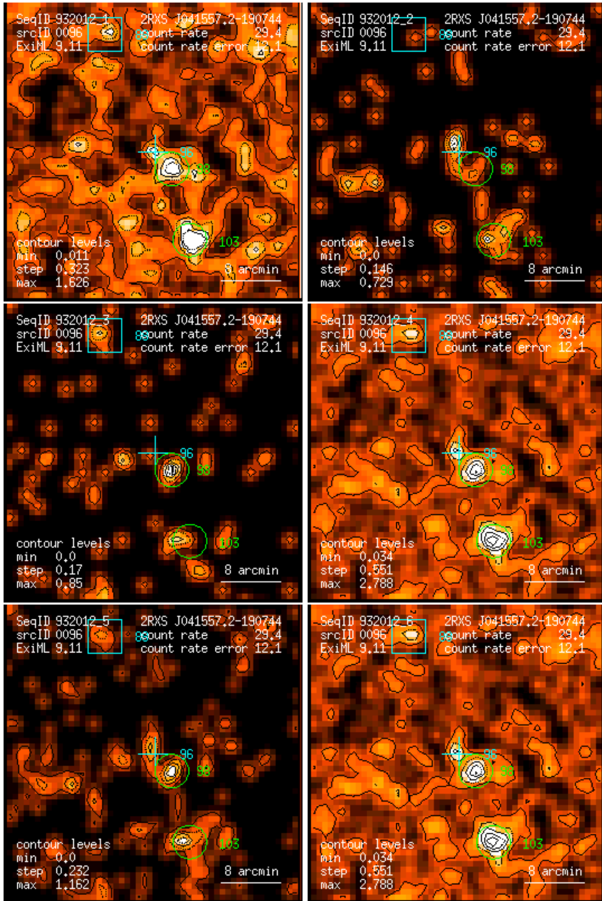
Figure 96: RASS 932012: detection 0096: band rate images, Gaussian filter: (1) PSPC channels 11 – 41, (2) 52 – 90, (3) 91 – 201, (4) 11 – 235, (5) 52 – 201, (6) 11 – 201. Broad band rates in counts/ks. Band rate contour levels in counts/ks/arcmin 2 .
