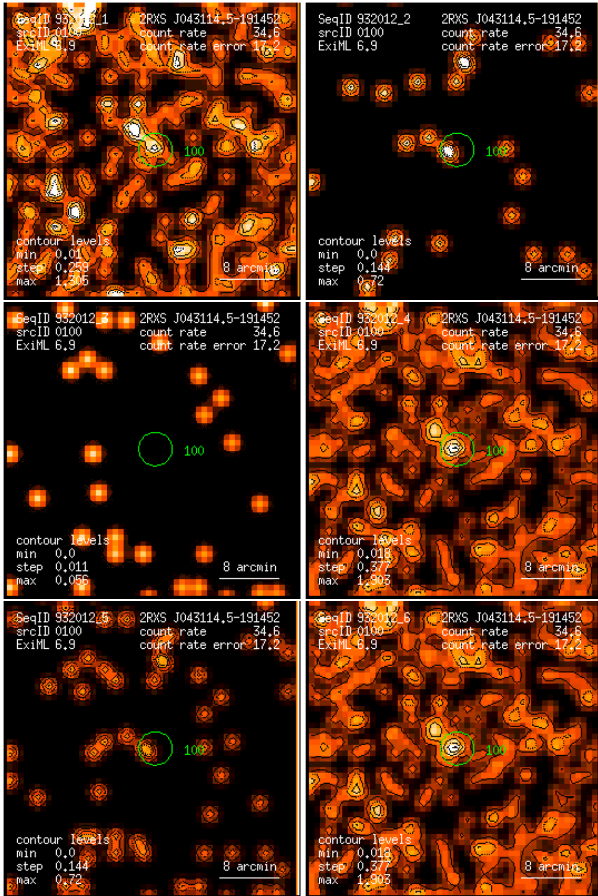
Figure 100: RASS 932012: detection 0100: band rate images, Gaussian filter: (1) PSPC channels 11 – 41, (2) 52 – 90, (3) 91 – 201, (4) 11 – 235, (5) 52 – 201, (6) 11 – 201. Broad band rates in counts/ks. Band rate contour levels in counts/ks/arcmin 2 .
