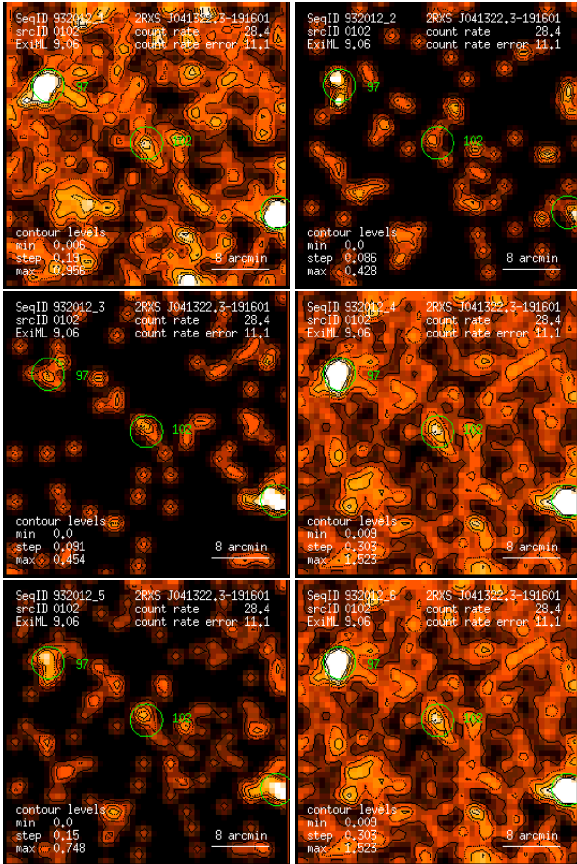
Figure 102: RASS 932012: detection 0102: band rate images, Gaussian filter: (1) PSPC channels 11 – 41, (2) 52 – 90, (3) 91 – 201, (4) 11 – 235, (5) 52 – 201, (6) 11 – 201. Broad band rates in counts/ks. Band rate contour levels in counts/ks/arcmin 2 .
