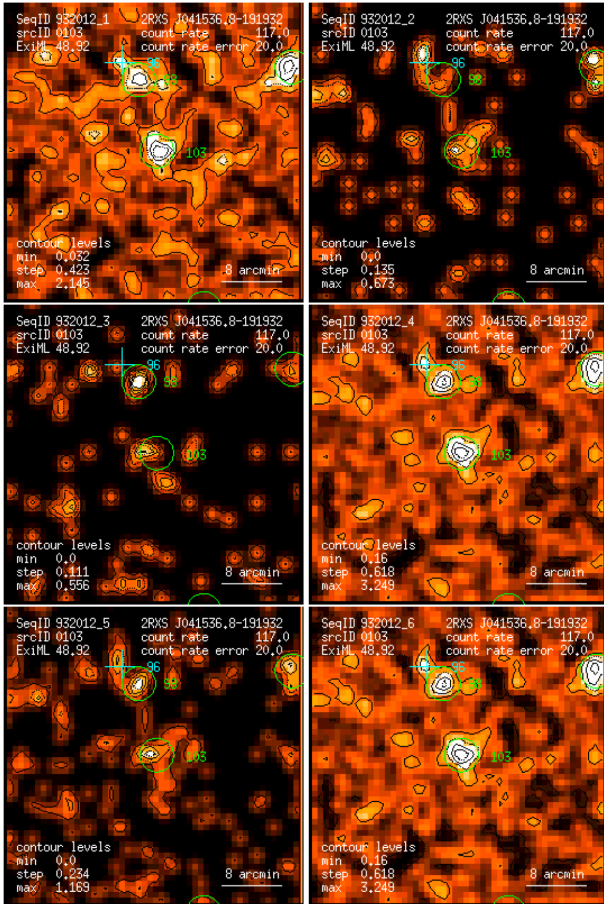
Figure 103: RASS 932012: detection 0103: band rate images, Gaussian filter: (1) PSPC channels 11 – 41, (2) 52 – 90, (3) 91 – 201, (4) 11 – 235, (5) 52 – 201, (6) 11 – 201. Broad band rates in counts/ks. Band rate contour levels in counts/ks/arcmin 2 .
