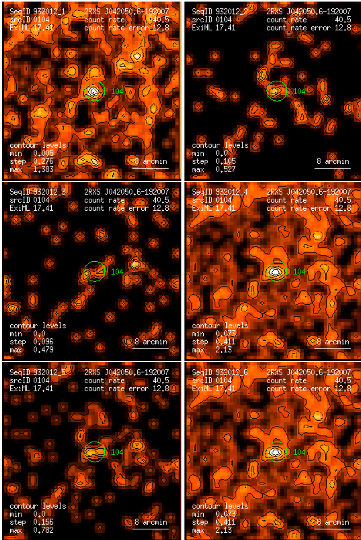
Figure 104: RASS 932012: detection 0104: band rate images, Gaussian filter: (1) PSPC channels 11 – 41, (2) 52 – 90, (3) 91 – 201, (4) 11 – 235, (5) 52 – 201, (6) 11 – 201. Broad band rates in counts/ks. Band rate contour levels in counts/ks/arcmin 2 .
