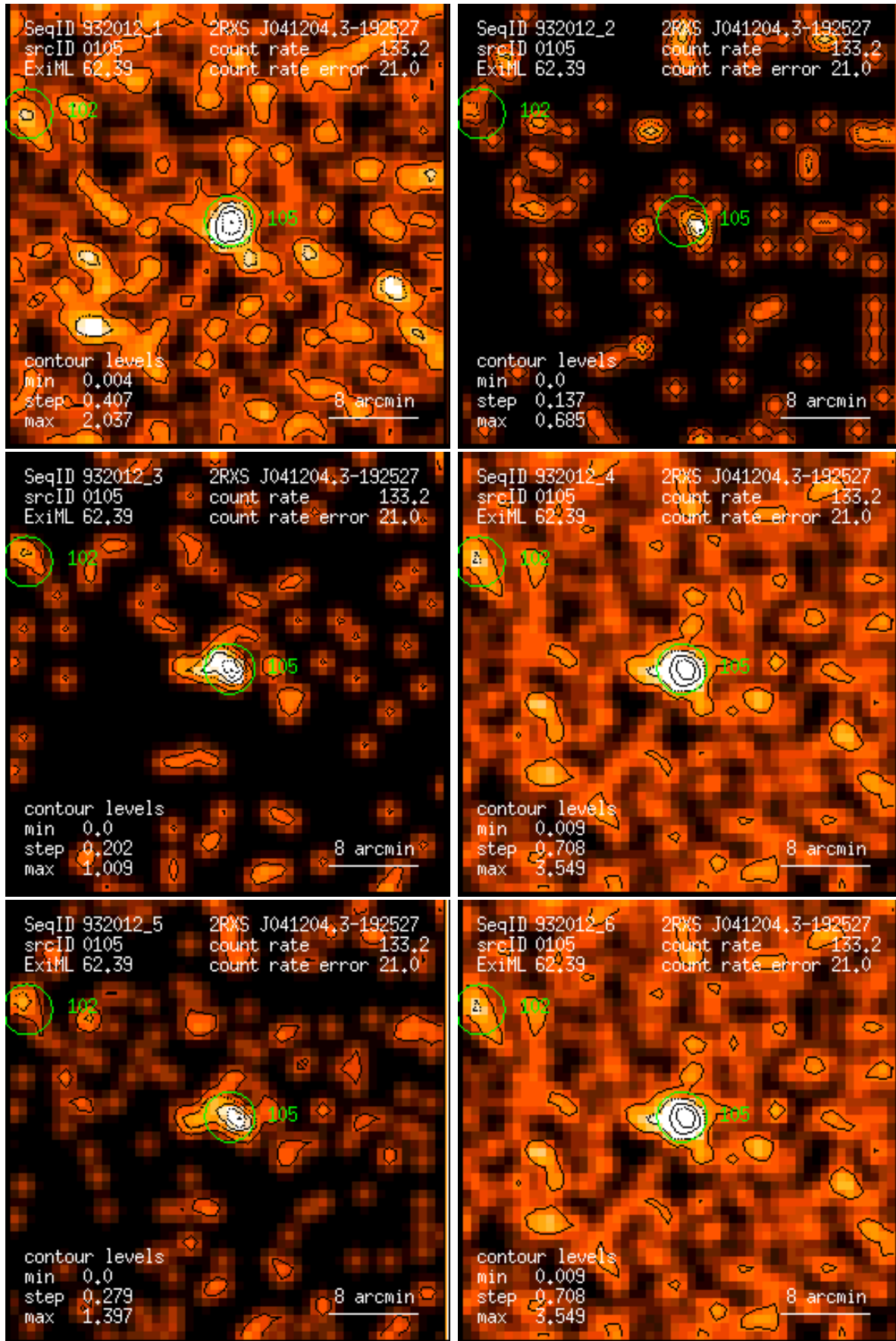
Figure 105: RASS 932012: detection 0105: band rate images, Gaussian filter: (1) PSPC channels 11 – 41, (2) 52 – 90, (3) 91 – 201, (4) 11 – 235, (5) 52 – 201, (6) 11 – 201. Broad band rates in counts/ks. Band rate contour levels in counts/ks/arcmin 2 .
