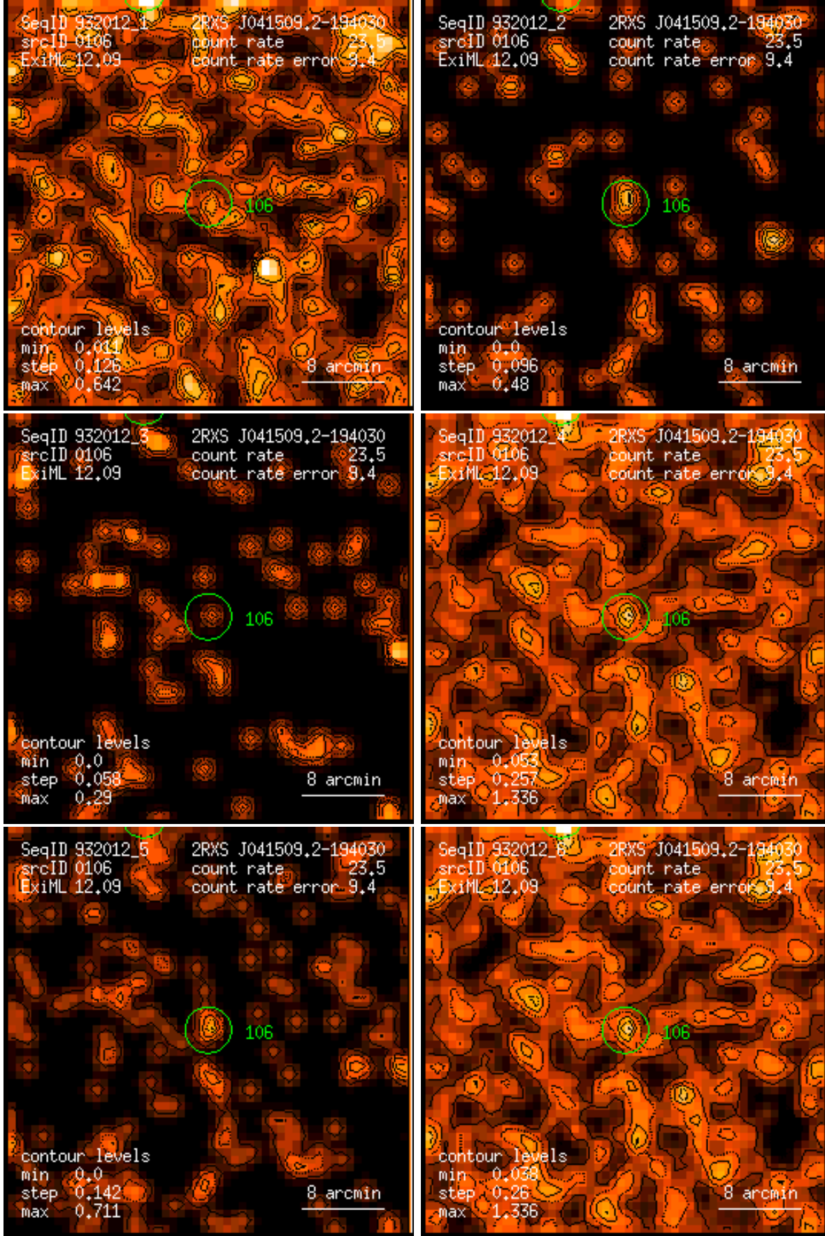
Figure 106: RASS 932012: detection 0106: band rate images, Gaussian filter: (1) PSPC channels 11 – 41, (2) 52 – 90, (3) 91 – 201, (4) 11 – 235, (5) 52 – 201, (6) 11 – 201. Broad band rates in counts/ks. Band rate contour levels in counts/ks/arcmin 2 .
