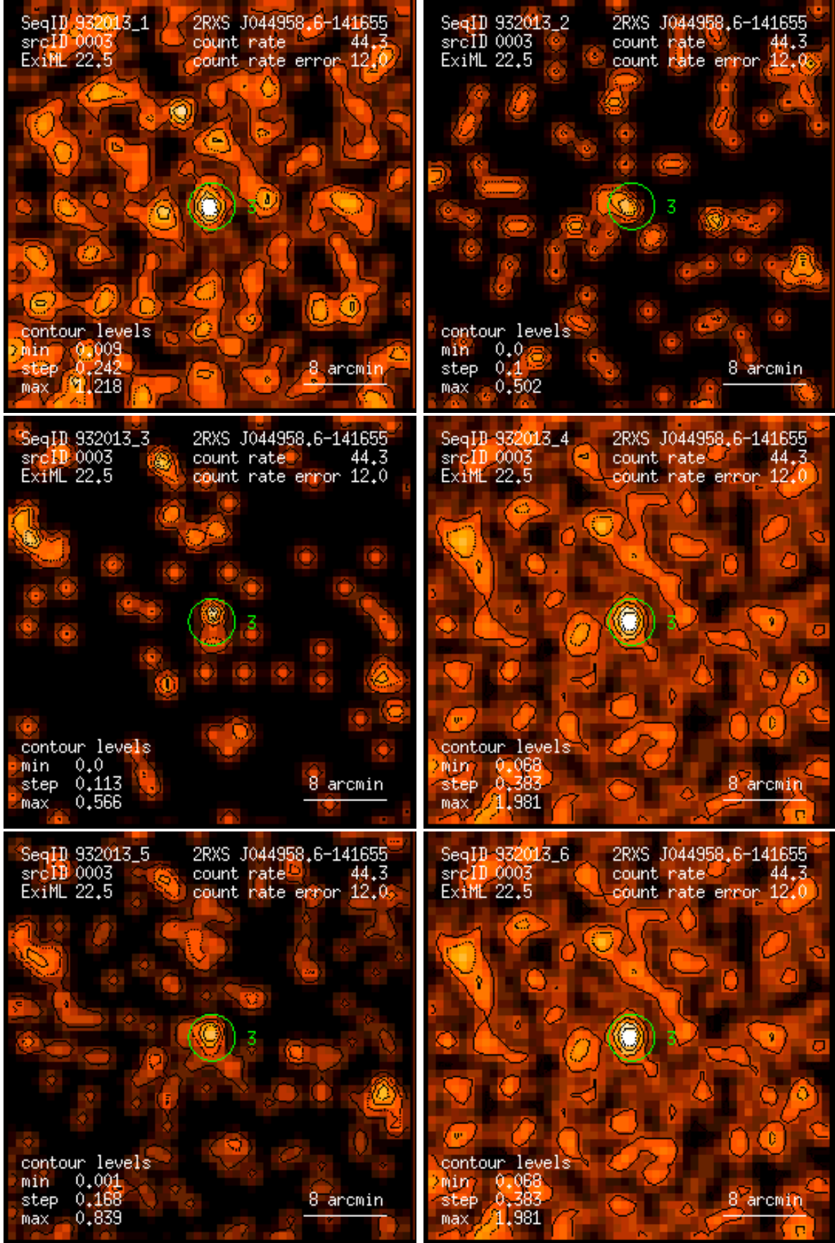
Figure 3: RASS 932013: detection 0003: band rate images, Gaussian filter: (1) PSPC channels 11 – 41, (2) 52 – 90, (3) 91 – 201, (4) 11 – 235, (5) 52 – 201, (6) 11 – 201. Broad band rates in counts/ks. Band rate contour levels in counts/ks/arcmin 2 .
