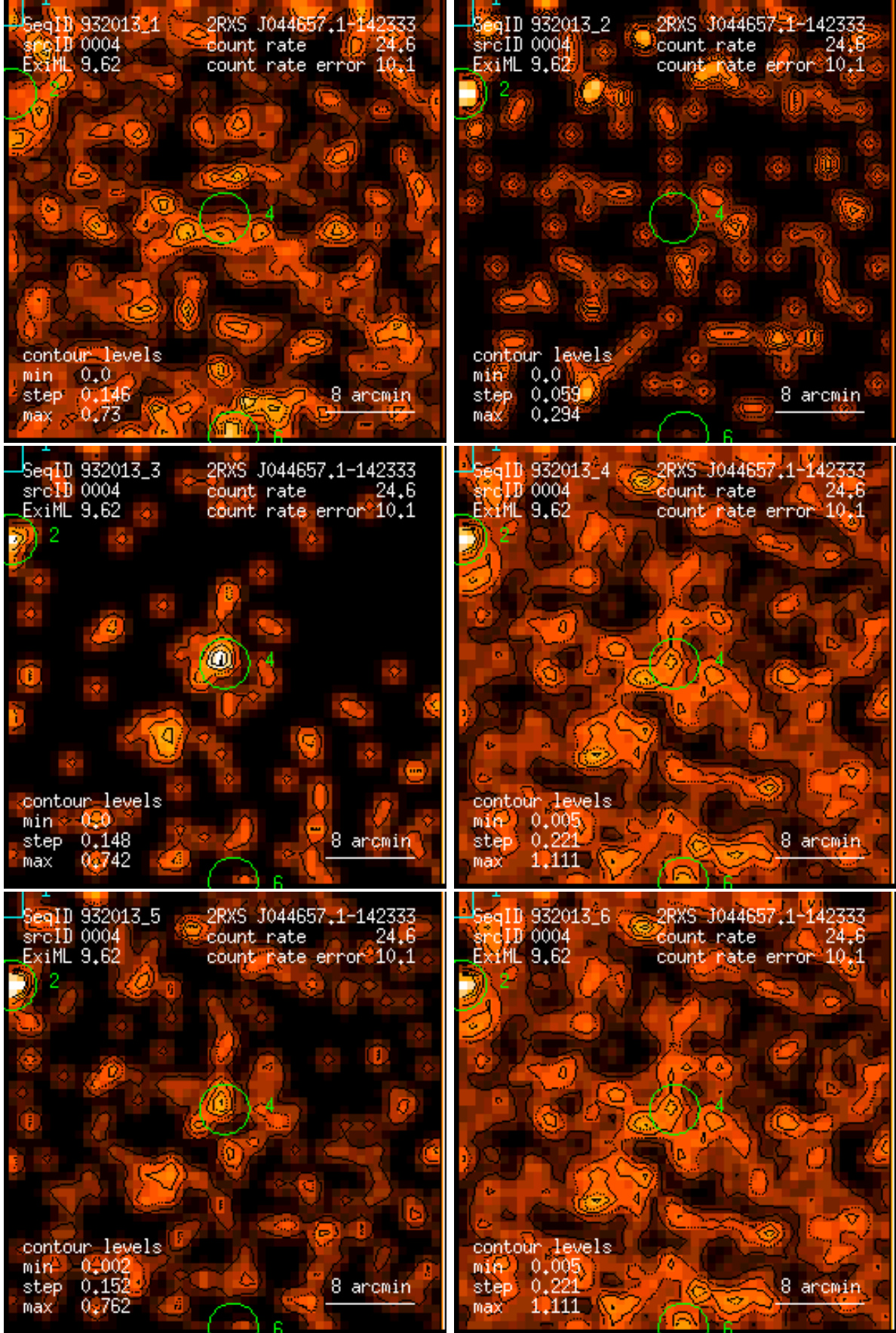
Figure 4: RASS 932013: detection 0004: band rate images, Gaussian filter: (1) PSPC channels 11 – 41, (2) 52 – 90, (3) 91 – 201, (4) 11 – 235, (5) 52 – 201, (6) 11 – 201. Broad band rates in counts/ks. Band rate contour levels in counts/ks/arcmin 2 .
