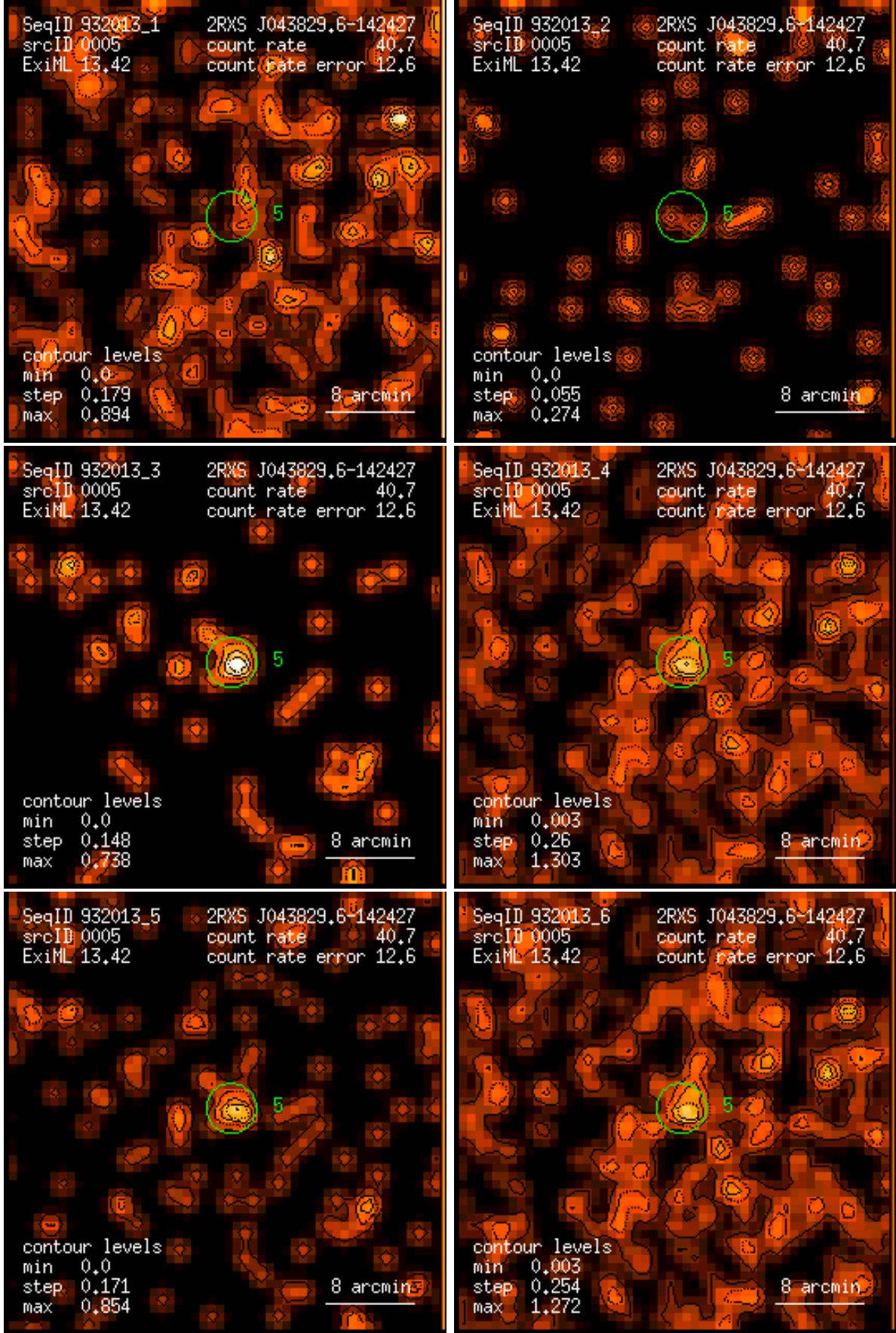
Figure 5: RASS 932013: detection 0005: band rate images, Gaussian filter: (1) PSPC channels 11 – 41, (2) 52 – 90, (3) 91 – 201, (4) 11 – 235, (5) 52 – 201, (6) 11 – 201. Broad band rates in counts/ks. Band rate contour levels in counts/ks/arcmin 2 .
